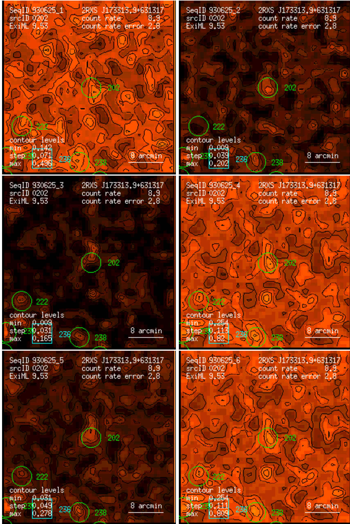
Figure 202: RASS 930625: detection 0202: band rate images, Gaussian filter: (1) PSPC channels 11 – 41, (2) 52 – 90, (3) 91 – 201, (4) 11 – 235, (5) 52 – 201, (6) 11 – 201. Broad band rates in counts/ks. Band rate contour levels in counts/ks/arcmin 2 .
