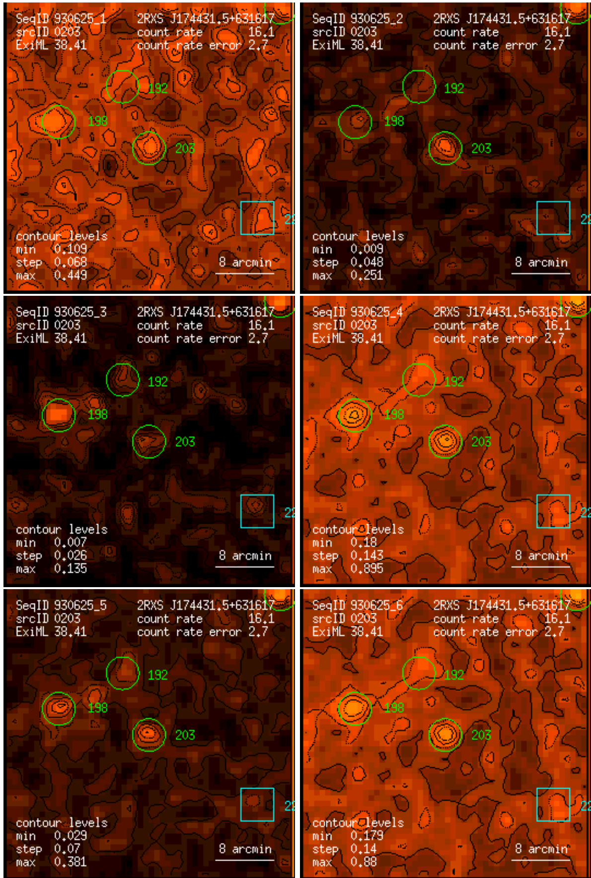
Figure 203: RASS 930625: detection 0203: band rate images, Gaussian filter: (1) PSPC channels 11 – 41, (2) 52 – 90, (3) 91 – 201, (4) 11 – 235, (5) 52 – 201, (6) 11 – 201. Broad band rates in counts/ks. Band rate contour levels in counts/ks/arcmin 2 .
