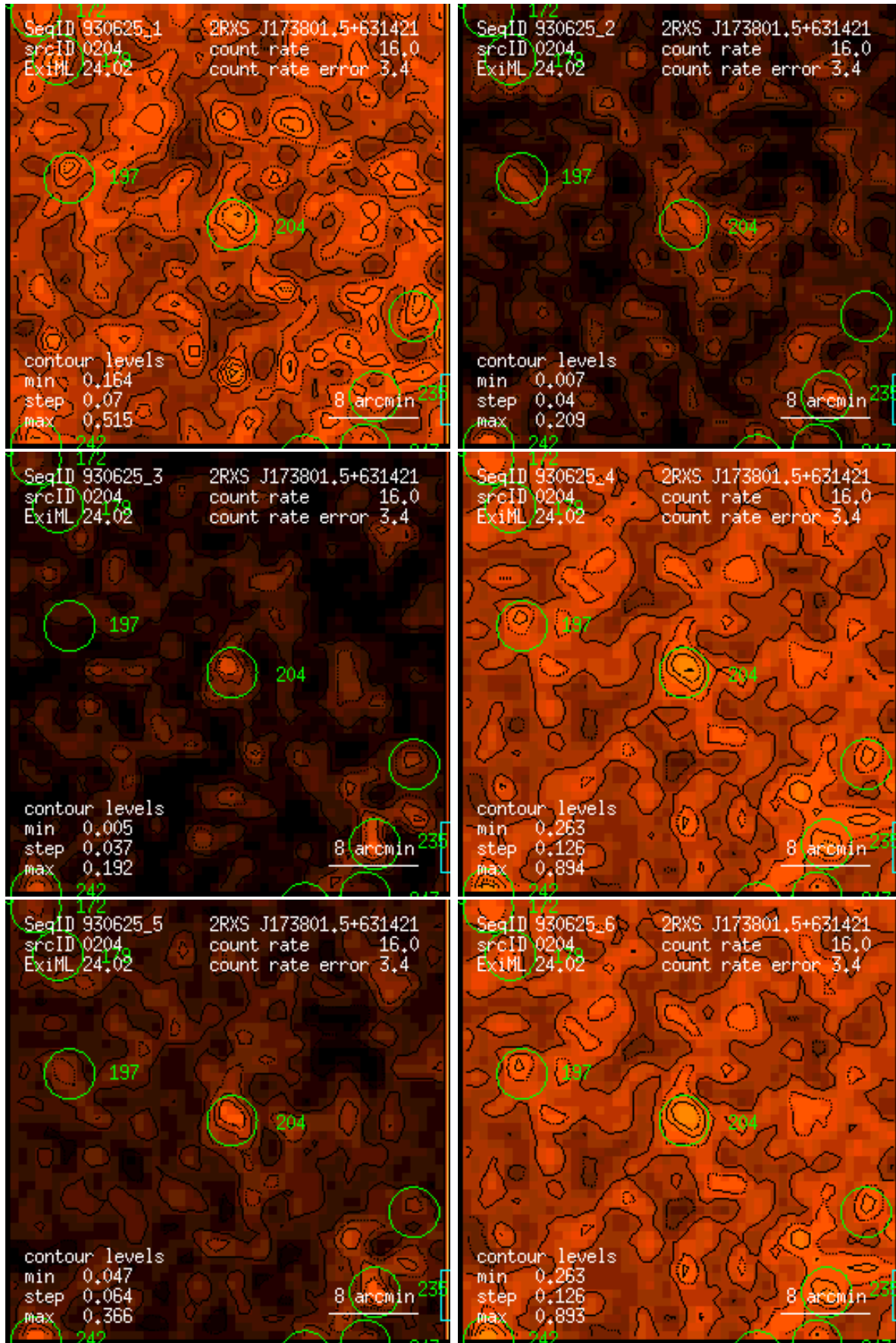
Figure 204: RASS 930625: detection 0204: band rate images, Gaussian filter: (1) PSPC channels 11 – 41, (2) 52 – 90, (3) 91 – 201, (4) 11 – 235, (5) 52 – 201, (6) 11 – 201. Broad band rates in counts/ks. Band rate contour levels in counts/ks/arcmin 2 .
