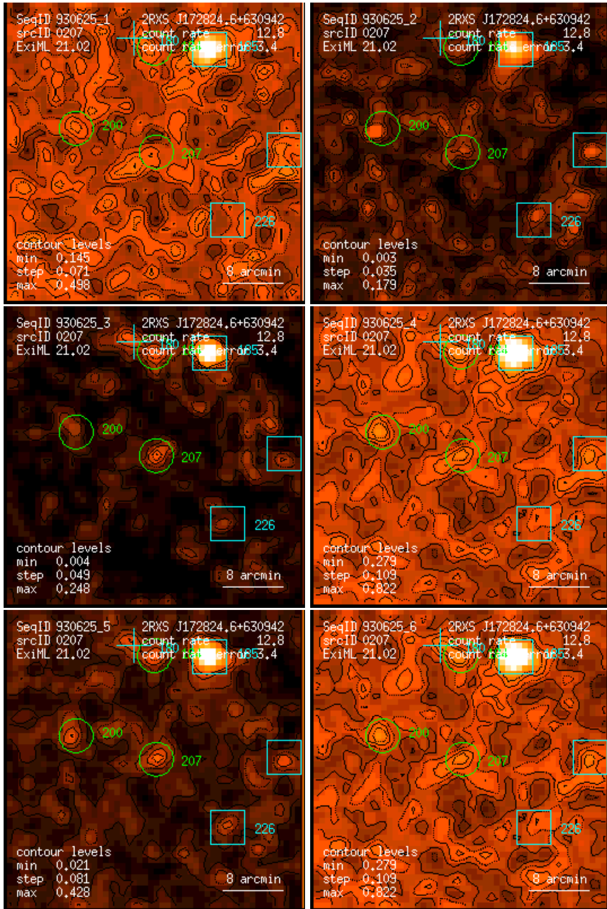
Figure 207: RASS 930625: detection 0207: band rate images, Gaussian filter: (1) PSPC channels 11 – 41, (2) 52 – 90, (3) 91 – 201, (4) 11 – 235, (5) 52 – 201, (6) 11 – 201. Broad band rates in counts/ks. Band rate contour levels in counts/ks/arcmin 2 .
