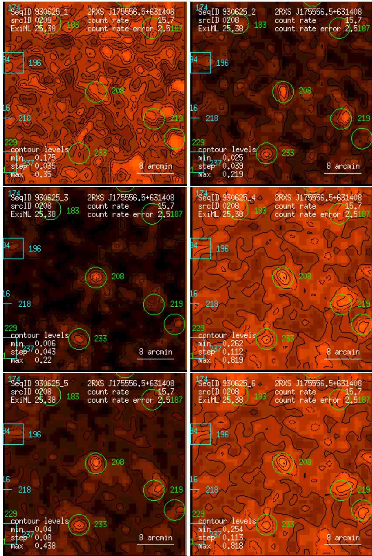
Figure 208: RASS 930625: detection 0208: band rate images, Gaussian filter: (1) PSPC channels 11 – 41, (2) 52 – 90, (3) 91 – 201, (4) 11 – 235, (5) 52 – 201, (6) 11 – 201. Broad band rates in counts/ks. Band rate contour levels in counts/ks/arcmin 2 .
