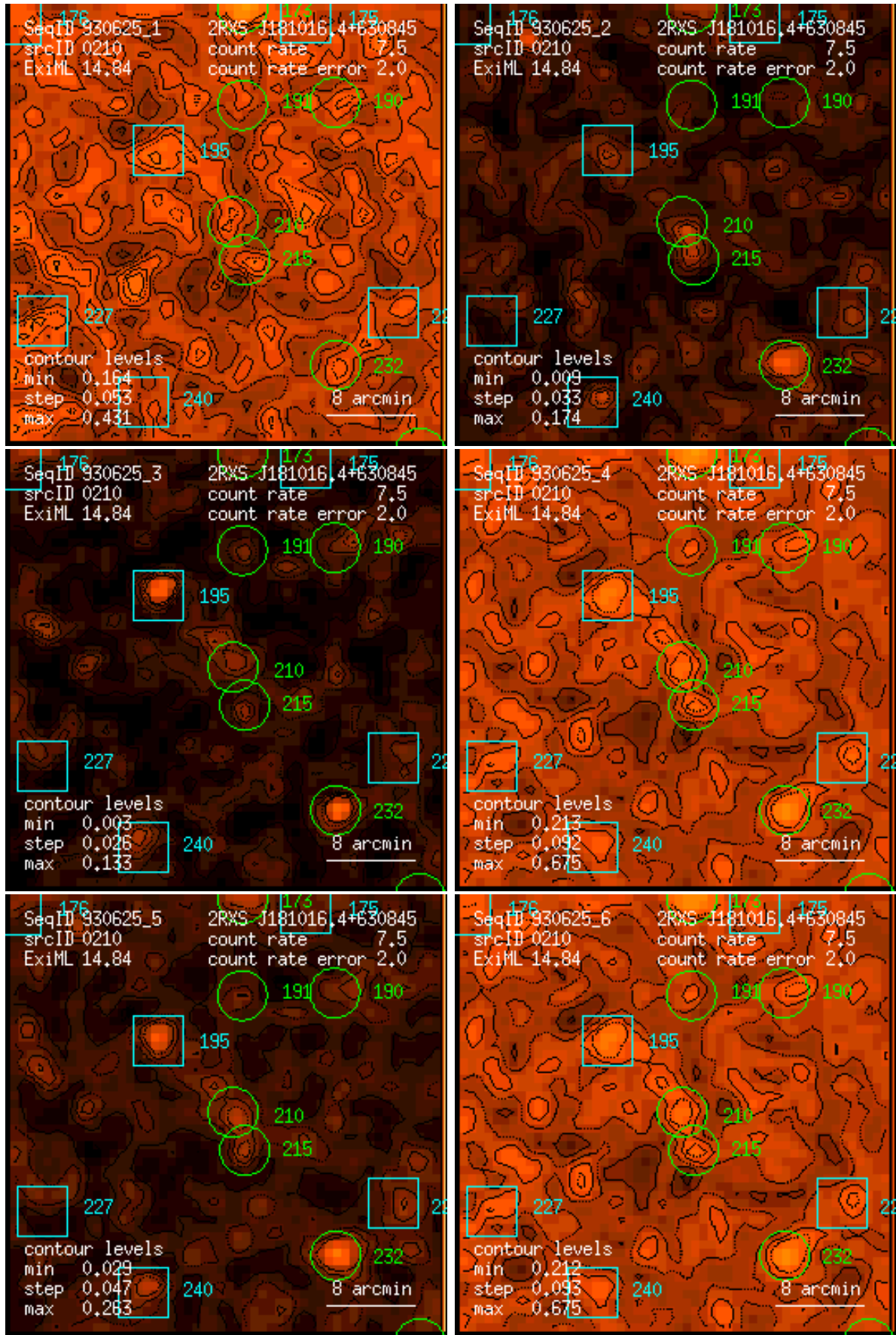
Figure 210: RASS 930625: detection 0210: band rate images, Gaussian filter: (1) PSPC channels 11 – 41, (2) 52 – 90, (3) 91 – 201, (4) 11 – 235, (5) 52 – 201, (6) 11 – 201. Broad band rates in counts/ks. Band rate contour levels in counts/ks/arcmin 2 .
