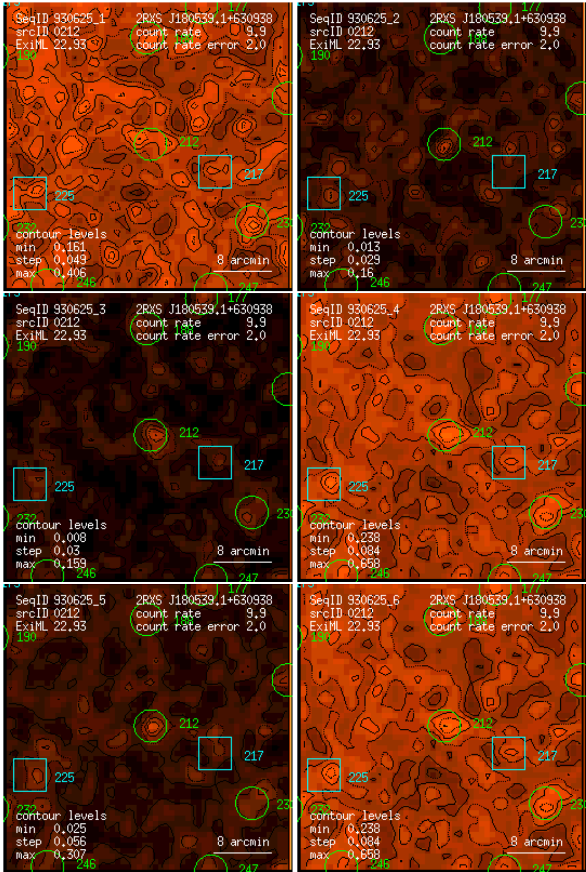
Figure 212: RASS 930625: detection 0212: band rate images, Gaussian filter: (1) PSPC channels 11 – 41, (2) 52 – 90, (3) 91 – 201, (4) 11 – 235, (5) 52 – 201, (6) 11 – 201. Broad band rates in counts/ks. Band rate contour levels in counts/ks/arcmin 2 .
