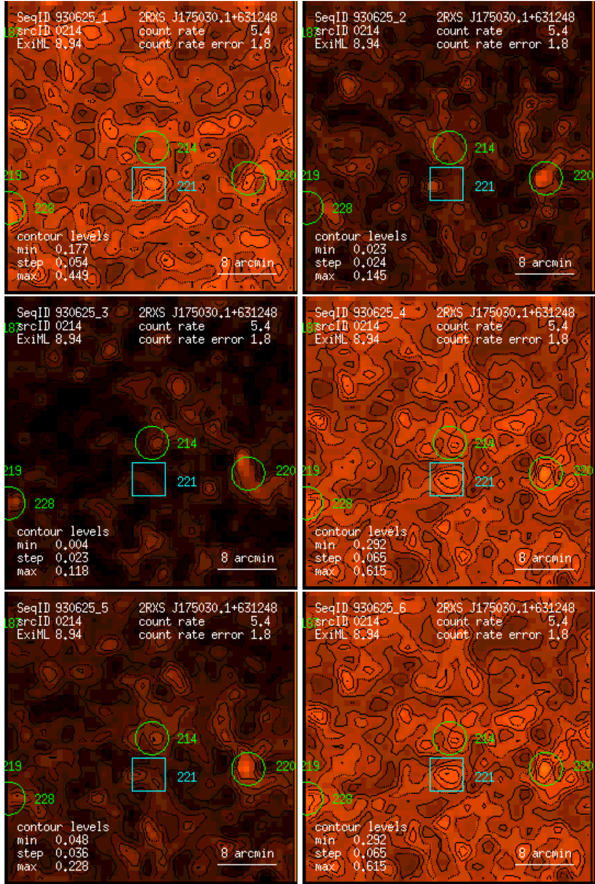
Figure 214: RASS 930625: detection 0214: band rate images, Gaussian filter: (1) PSPC channels 11 – 41, (2) 52 – 90, (3) 91 – 201, (4) 11 – 235, (5) 52 – 201, (6) 11 – 201. Broad band rates in counts/ks. Band rate contour levels in counts/ks/arcmin 2 .
