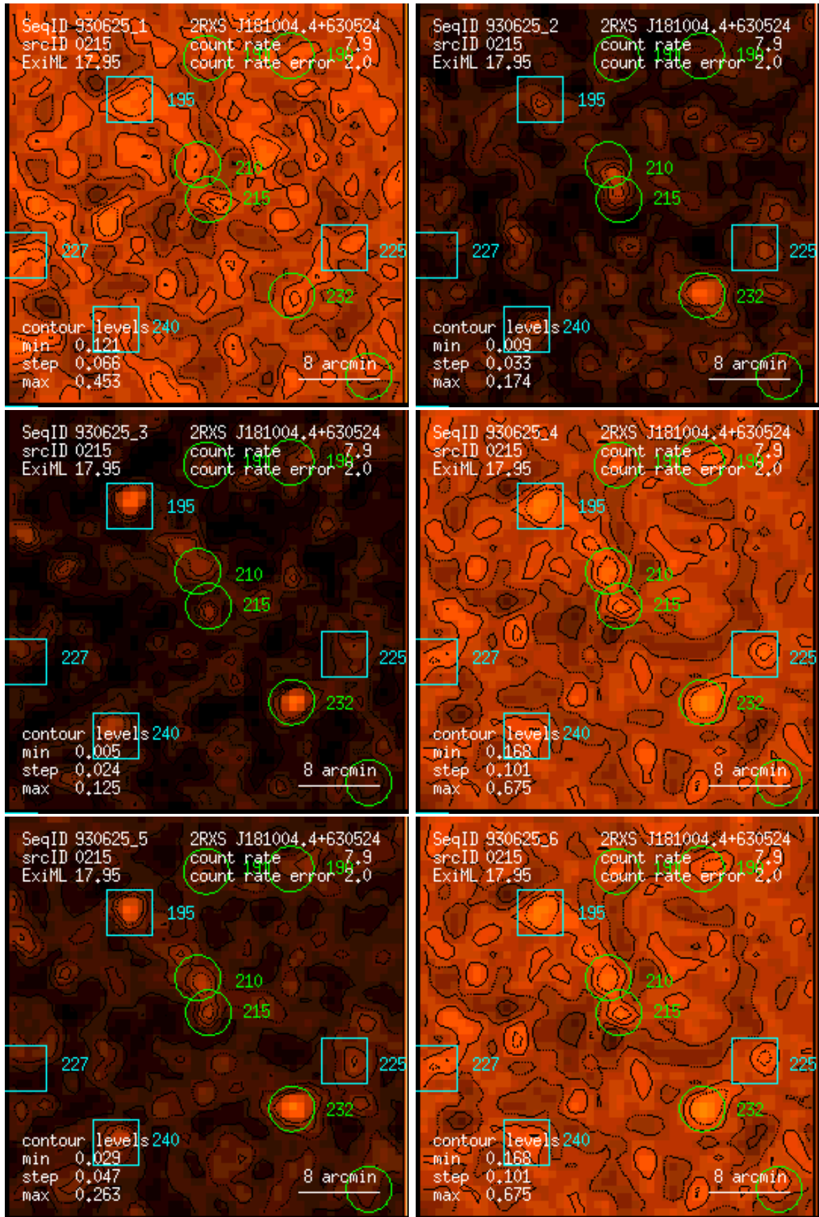
Figure 215: RASS 930625: detection 0215: band rate images, Gaussian filter: (1) PSPC channels 11 – 41, (2) 52 – 90, (3) 91 – 201, (4) 11 – 235, (5) 52 – 201, (6) 11 – 201. Broad band rates in counts/ks. Band rate contour levels in counts/ks/arcmin 2 .
