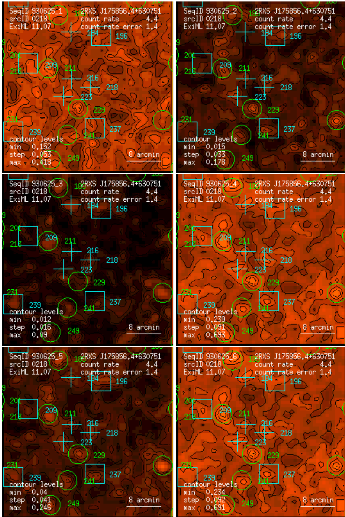
Figure 218: RASS 930625: detection 0218: band rate images, Gaussian filter: (1) PSPC channels 11 – 41, (2) 52 – 90, (3) 91 – 201, (4) 11 – 235, (5) 52 – 201, (6) 11 – 201. Broad band rates in counts/ks. Band rate contour levels in counts/ks/arcmin 2 .
