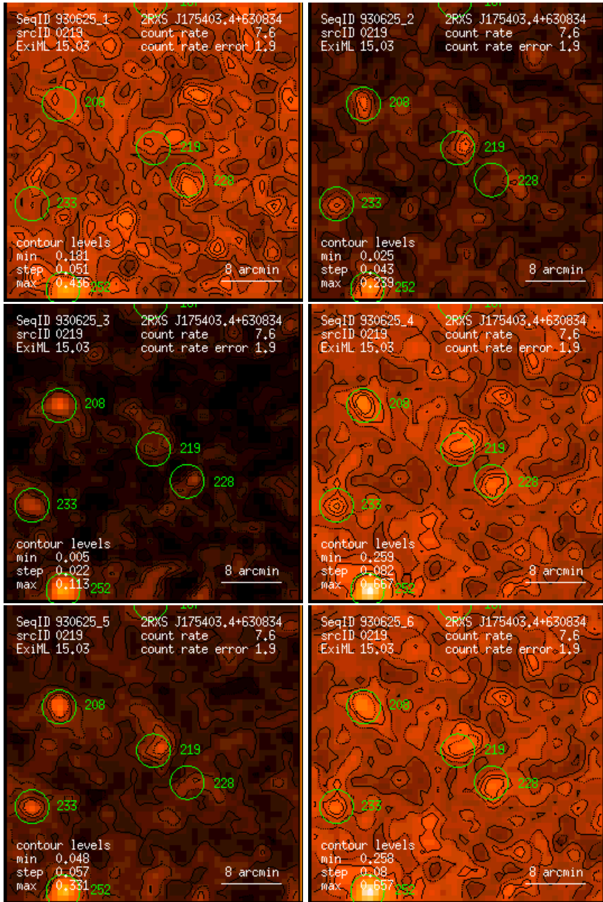
Figure 219: RASS 930625: detection 0219: band rate images, Gaussian filter: (1) PSPC channels 11 – 41, (2) 52 – 90, (3) 91 – 201, (4) 11 – 235, (5) 52 – 201, (6) 11 – 201. Broad band rates in counts/ks. Band rate contour levels in counts/ks/arcmin 2 .
