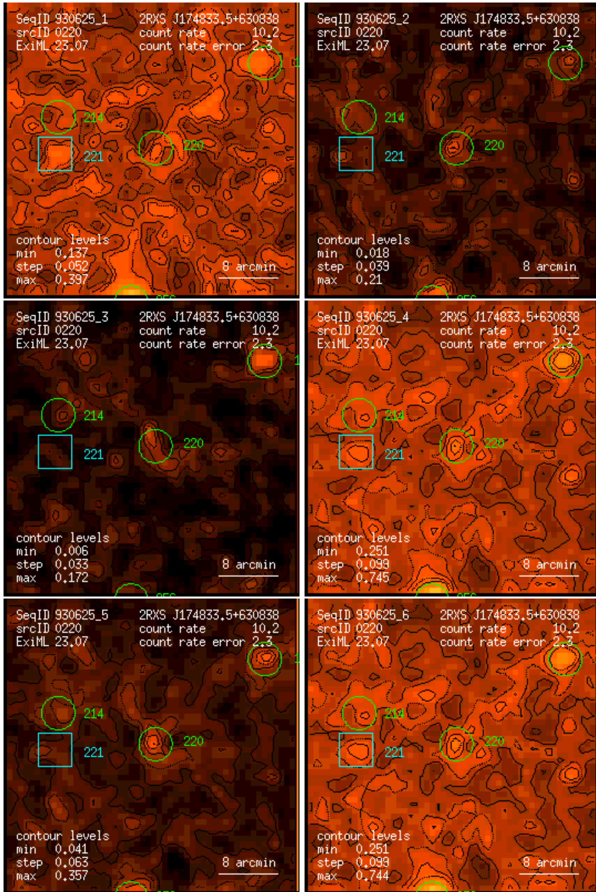
Figure 220: RASS 930625: detection 0220: band rate images, Gaussian filter: (1) PSPC channels 11 – 41, (2) 52 – 90, (3) 91 – 201, (4) 11 – 235, (5) 52 – 201, (6) 11 – 201. Broad band rates in counts/ks. Band rate contour levels in counts/ks/arcmin 2 .
