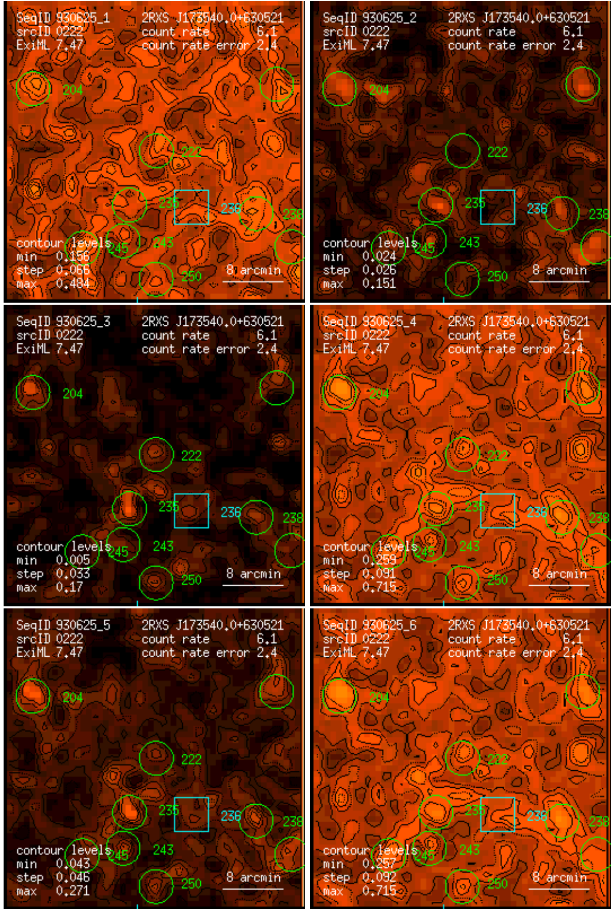
Figure 222: RASS 930625: detection 0222: band rate images, Gaussian filter: (1) PSPC channels 11 – 41, (2) 52 – 90, (3) 91 – 201, (4) 11 – 235, (5) 52 – 201, (6) 11 – 201. Broad band rates in counts/ks. Band rate contour levels in counts/ks/arcmin 2 .
