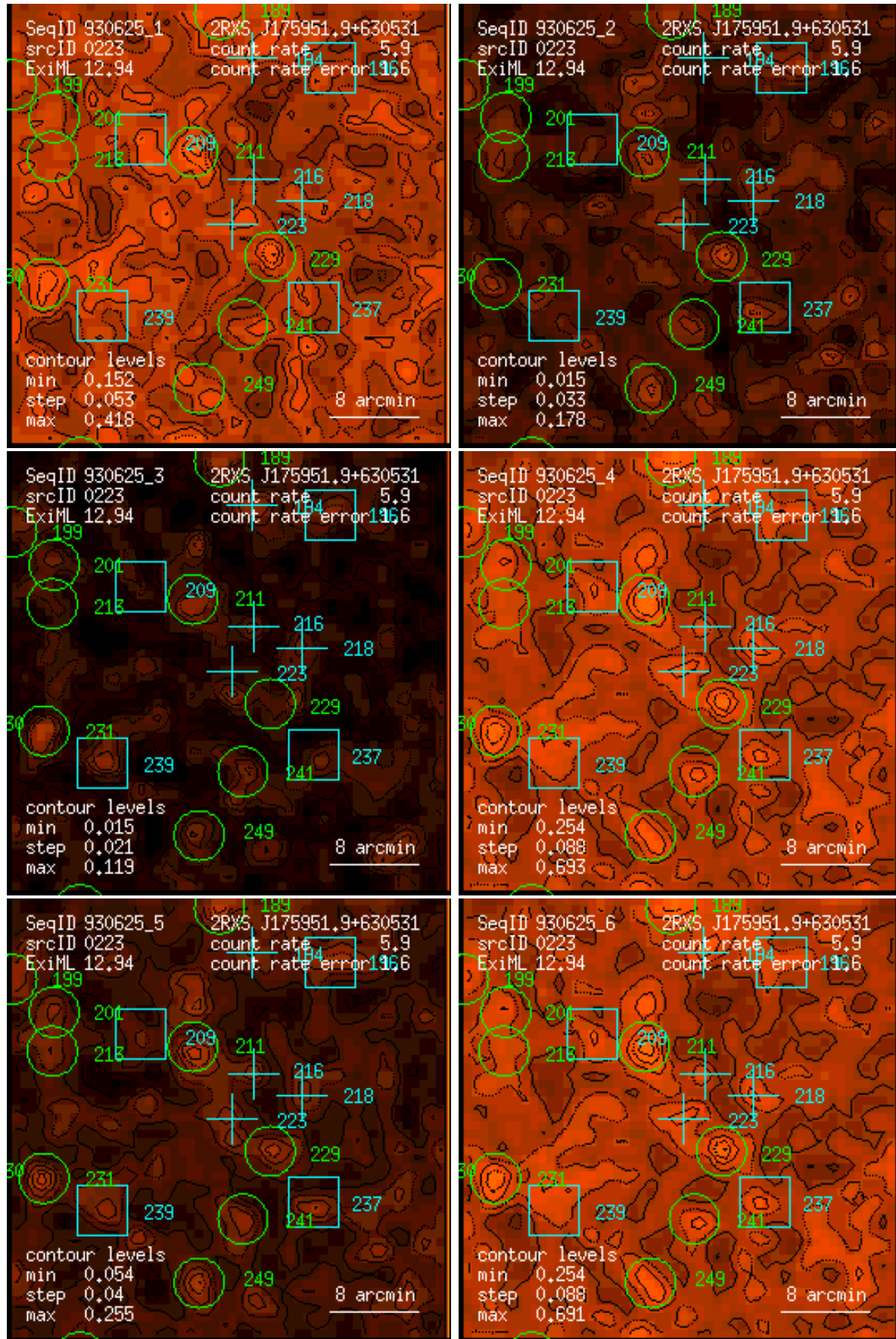
Figure 223: RASS 930625: detection 0223: band rate images, Gaussian filter: (1) PSPC channels 11 – 41, (2) 52 – 90, (3) 91 – 201, (4) 11 – 235, (5) 52 – 201, (6) 11 – 201. Broad band rates in counts/ks. Band rate contour levels in counts/ks/arcmin 2 .
