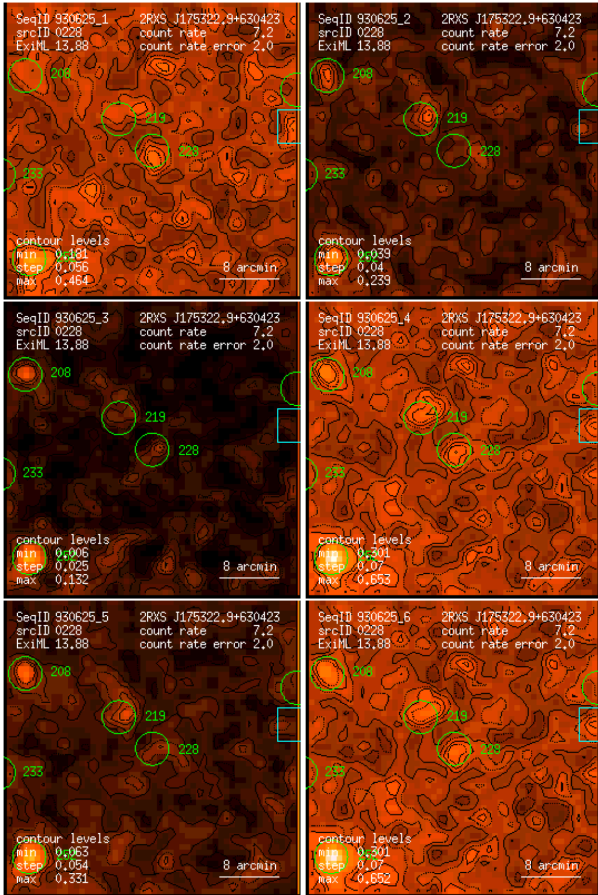
Figure 228: RASS 930625: detection 0228: band rate images, Gaussian filter: (1) PSPC channels 11 – 41, (2) 52 – 90, (3) 91 – 201, (4) 11 – 235, (5) 52 – 201, (6) 11 – 201. Broad band rates in counts/ks. Band rate contour levels in counts/ks/arcmin 2 .
