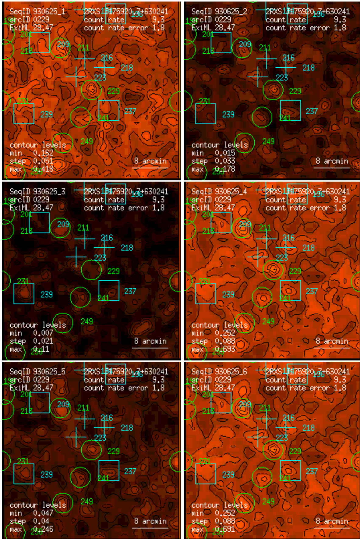
Figure 229: RASS 930625: detection 0229: band rate images, Gaussian filter: (1) PSPC channels 11 – 41, (2) 52 – 90, (3) 91 – 201, (4) 11 – 235, (5) 52 – 201, (6) 11 – 201. Broad band rates in counts/ks. Band rate contour levels in counts/ks/arcmin 2 .
