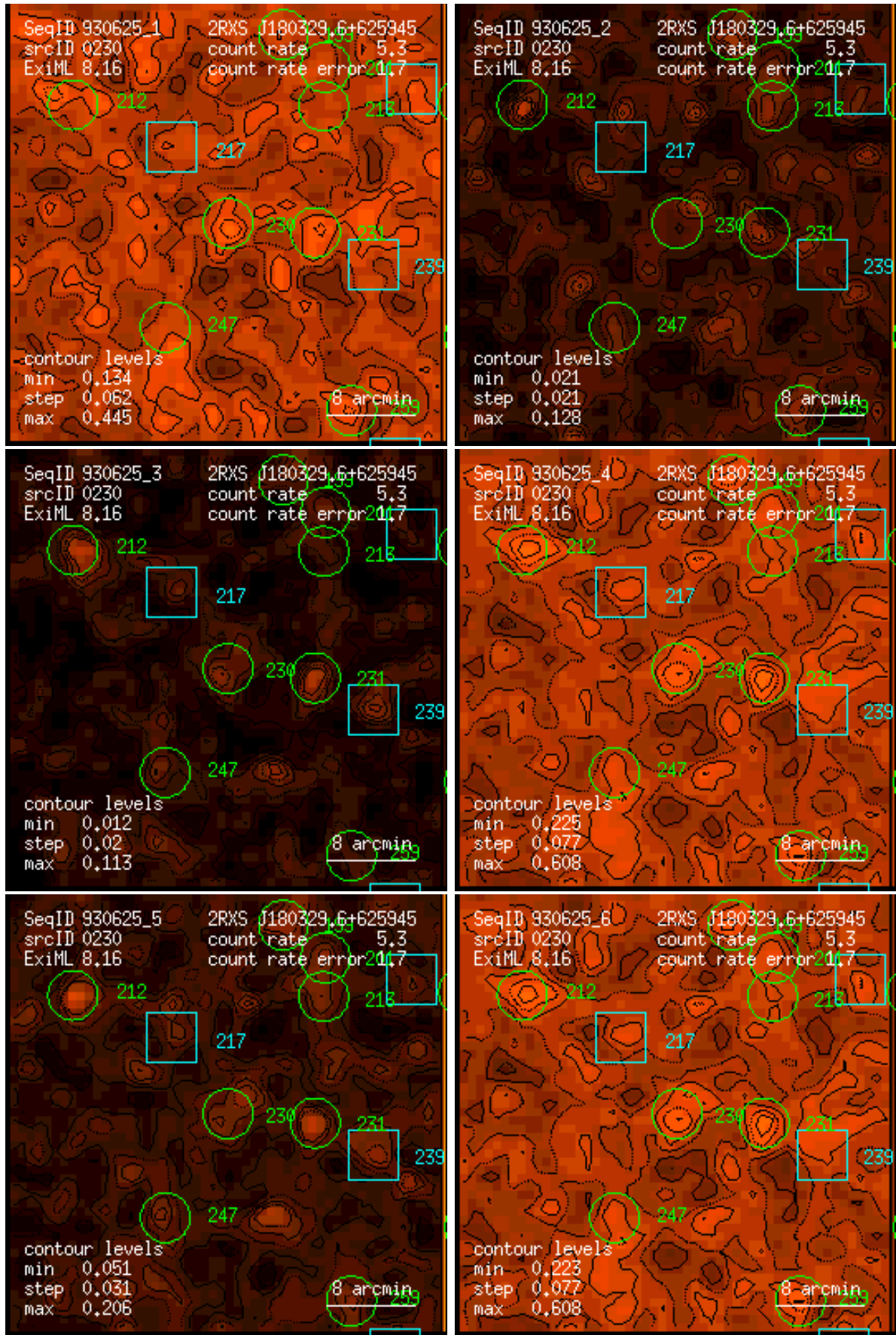
Figure 230: RASS 930625: detection 0230: band rate images, Gaussian filter: (1) PSPC channels 11 – 41, (2) 52 – 90, (3) 91 – 201, (4) 11 – 235, (5) 52 – 201, (6) 11 – 201. Broad band rates in counts/ks. Band rate contour levels in counts/ks/arcmin 2 .
