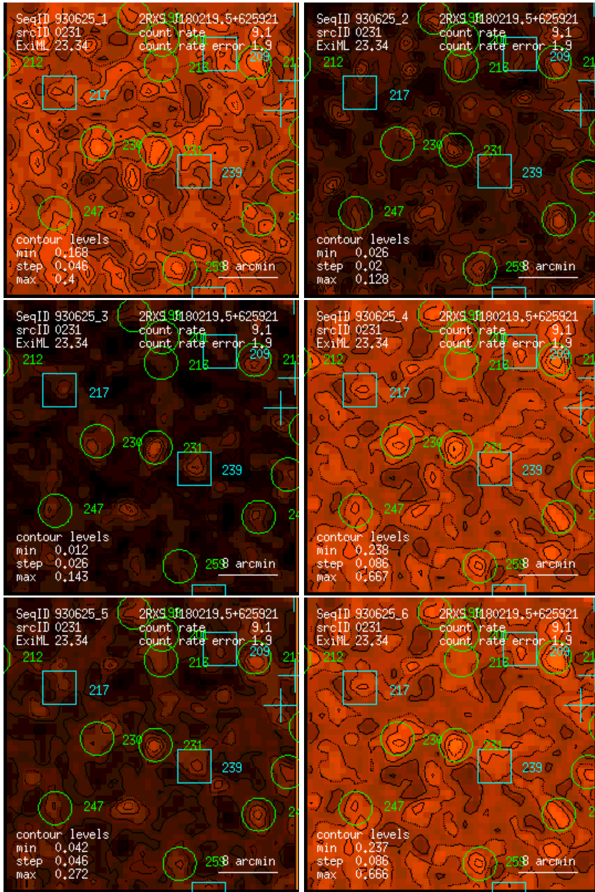
Figure 231: RASS 930625: detection 0231: band rate images, Gaussian filter: (1) PSPC channels 11 – 41, (2) 52 – 90, (3) 91 – 201, (4) 11 – 235, (5) 52 – 201, (6) 11 – 201. Broad band rates in counts/ks. Band rate contour levels in counts/ks/arcmin 2 .
