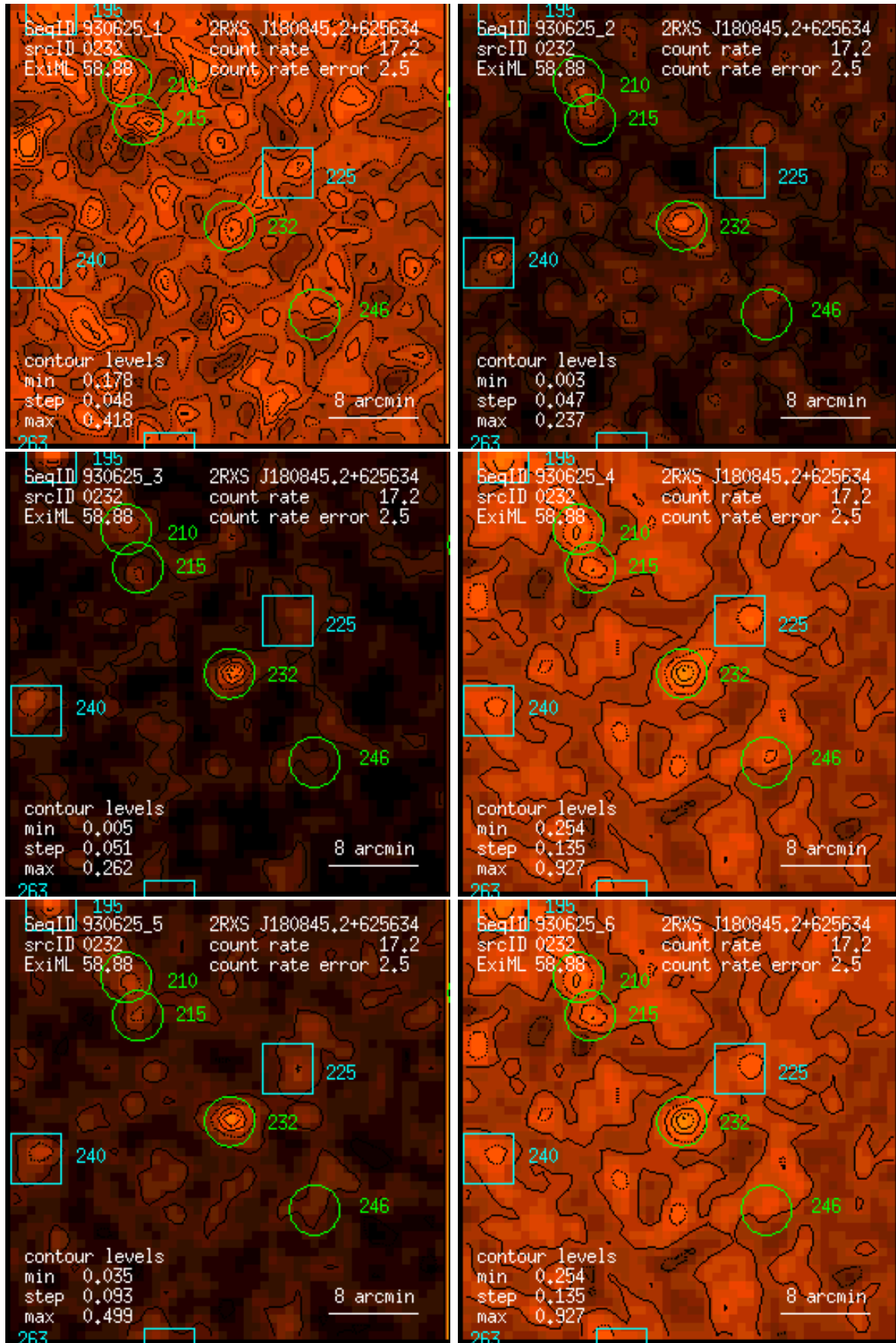
Figure 232: RASS 930625: detection 0232: band rate images, Gaussian filter: (1) PSPC channels 11 – 41, (2) 52 – 90, (3) 91 – 201, (4) 11 – 235, (5) 52 – 201, (6) 11 – 201. Broad band rates in counts/ks. Band rate contour levels in counts/ks/arcmin 2 .
