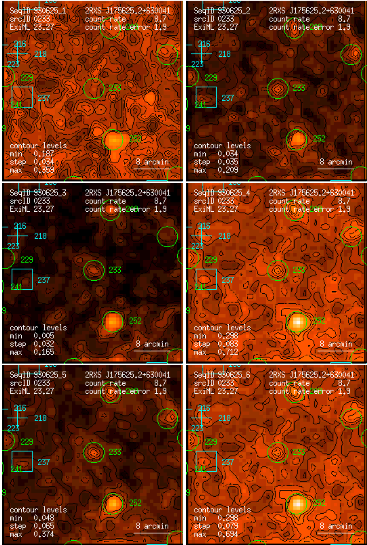
Figure 233: RASS 930625: detection 0233: band rate images, Gaussian filter: (1) PSPC channels 11 – 41, (2) 52 – 90, (3) 91 – 201, (4) 11 – 235, (5) 52 – 201, (6) 11 – 201. Broad band rates in counts/ks. Band rate contour levels in counts/ks/arcmin 2 .
