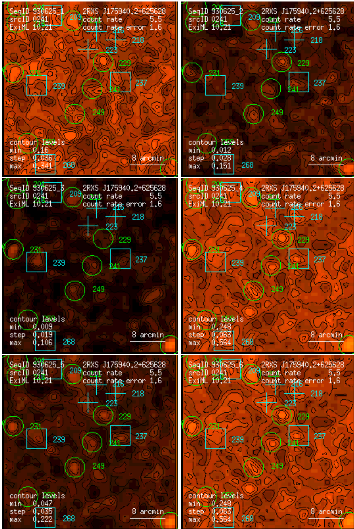
Figure 241: RASS 930625: detection 0241: band rate images, Gaussian filter: (1) PSPC channels 11 – 41, (2) 52 – 90, (3) 91 – 201, (4) 11 – 235, (5) 52 – 201, (6) 11 – 201. Broad band rates in counts/ks. Band rate contour levels in counts/ks/arcmin 2 .
