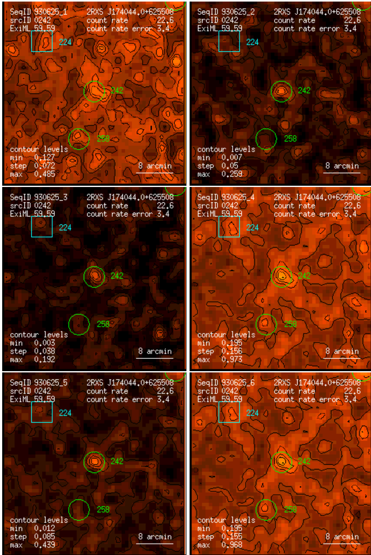
Figure 242: RASS 930625: detection 0242: band rate images, Gaussian filter: (1) PSPC channels 11 – 41, (2) 52 – 90, (3) 91 – 201, (4) 11 – 235, (5) 52 – 201, (6) 11 – 201. Broad band rates in counts/ks. Band rate contour levels in counts/ks/arcmin 2 .
