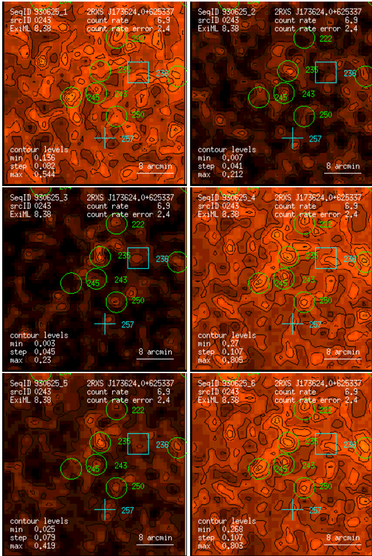
Figure 243: RASS 930625: detection 0243: band rate images, Gaussian filter: (1) PSPC channels 11 – 41, (2) 52 – 90, (3) 91 – 201, (4) 11 – 235, (5) 52 – 201, (6) 11 – 201. Broad band rates in counts/ks. Band rate contour levels in counts/ks/arcmin 2 .
