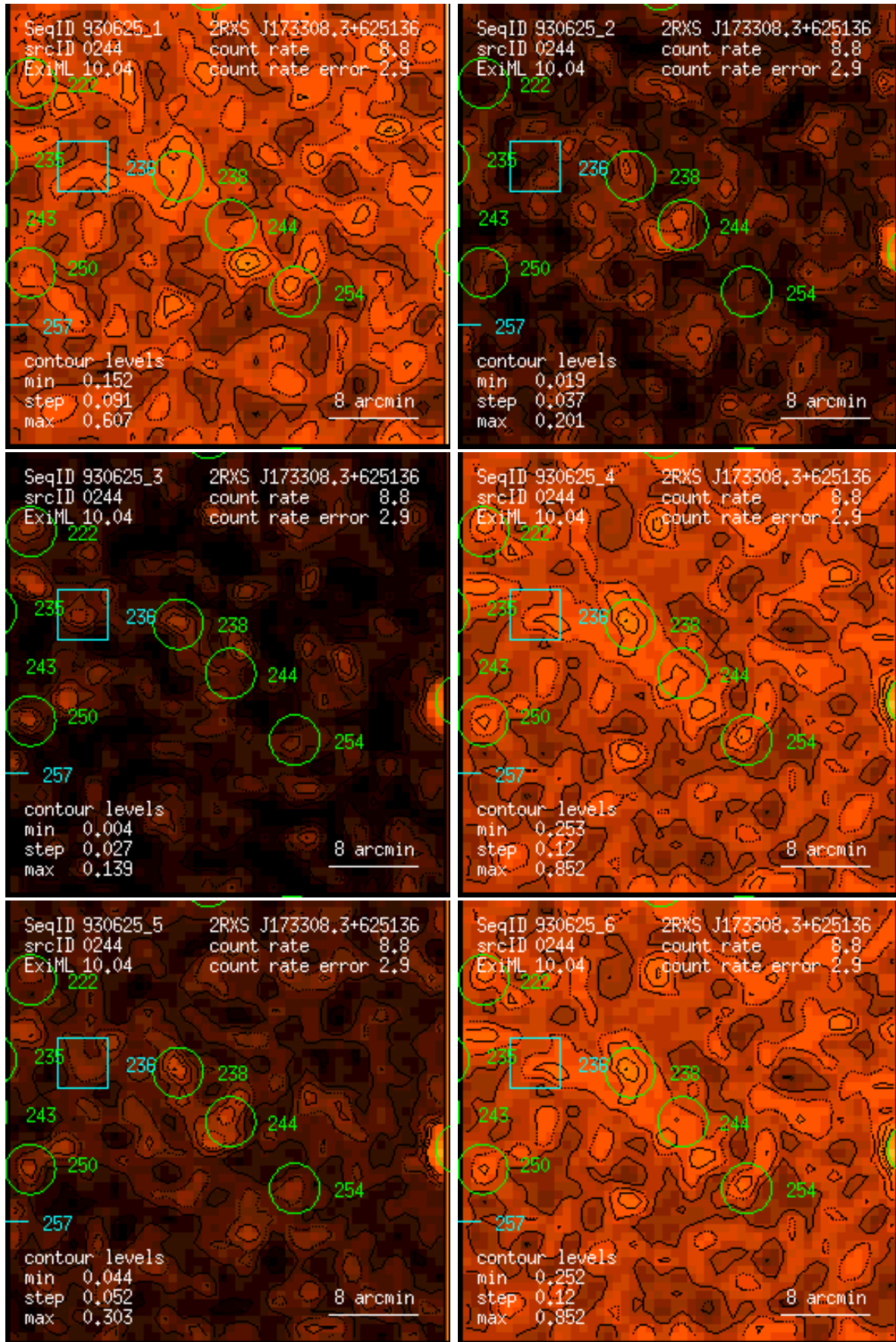
Figure 244: RASS 930625: detection 0244: band rate images, Gaussian filter: (1) PSPC channels 11 – 41, (2) 52 – 90, (3) 91 – 201, (4) 11 – 235, (5) 52 – 201, (6) 11 – 201. Broad band rates in counts/ks. Band rate contour levels in counts/ks/arcmin 2 .
