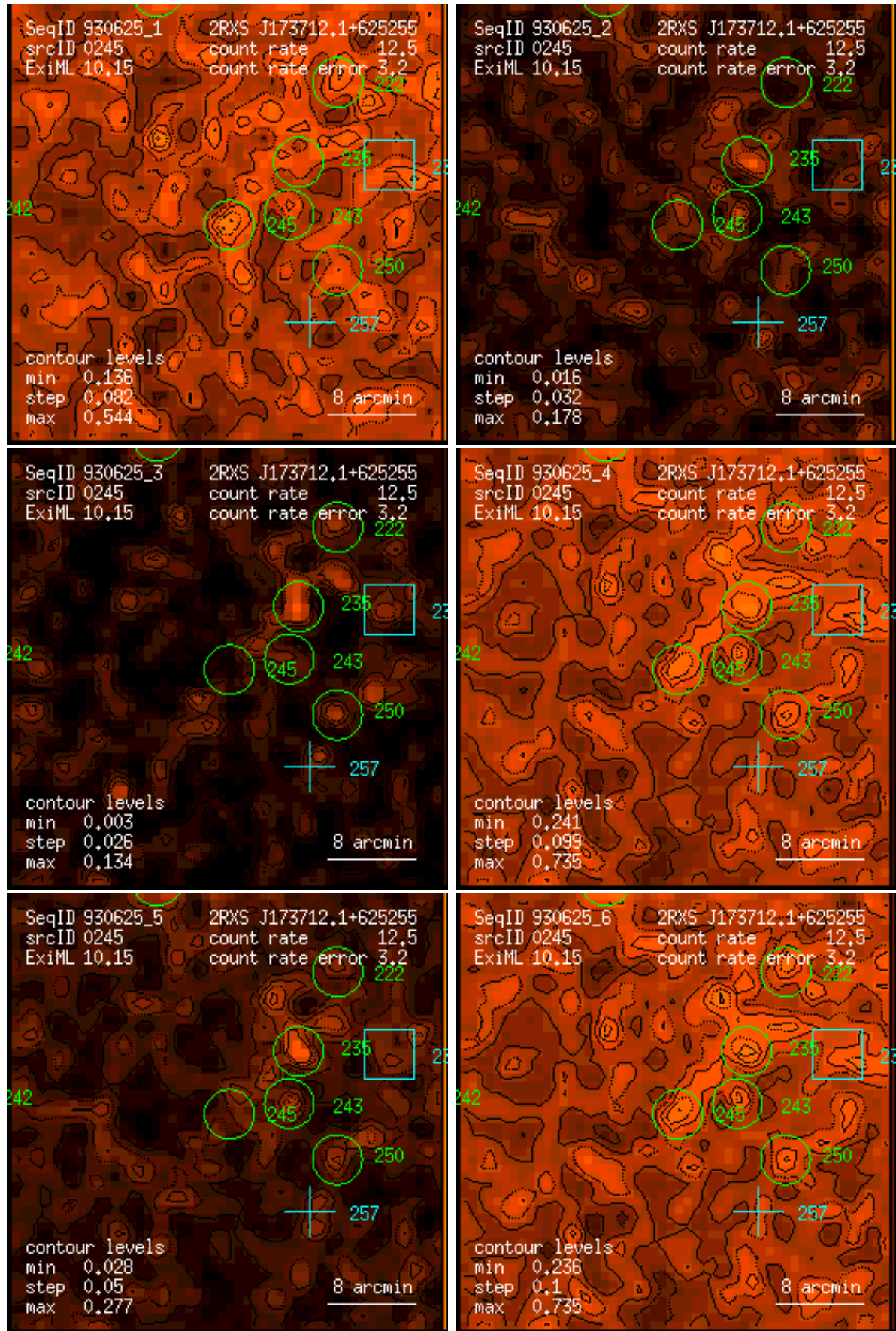
Figure 245: RASS 930625: detection 0245: band rate images, Gaussian filter: (1) PSPC channels 11 – 41, (2) 52 – 90, (3) 91 – 201, (4) 11 – 235, (5) 52 – 201, (6) 11 – 201. Broad band rates in counts/ks. Band rate contour levels in counts/ks/arcmin 2 .
