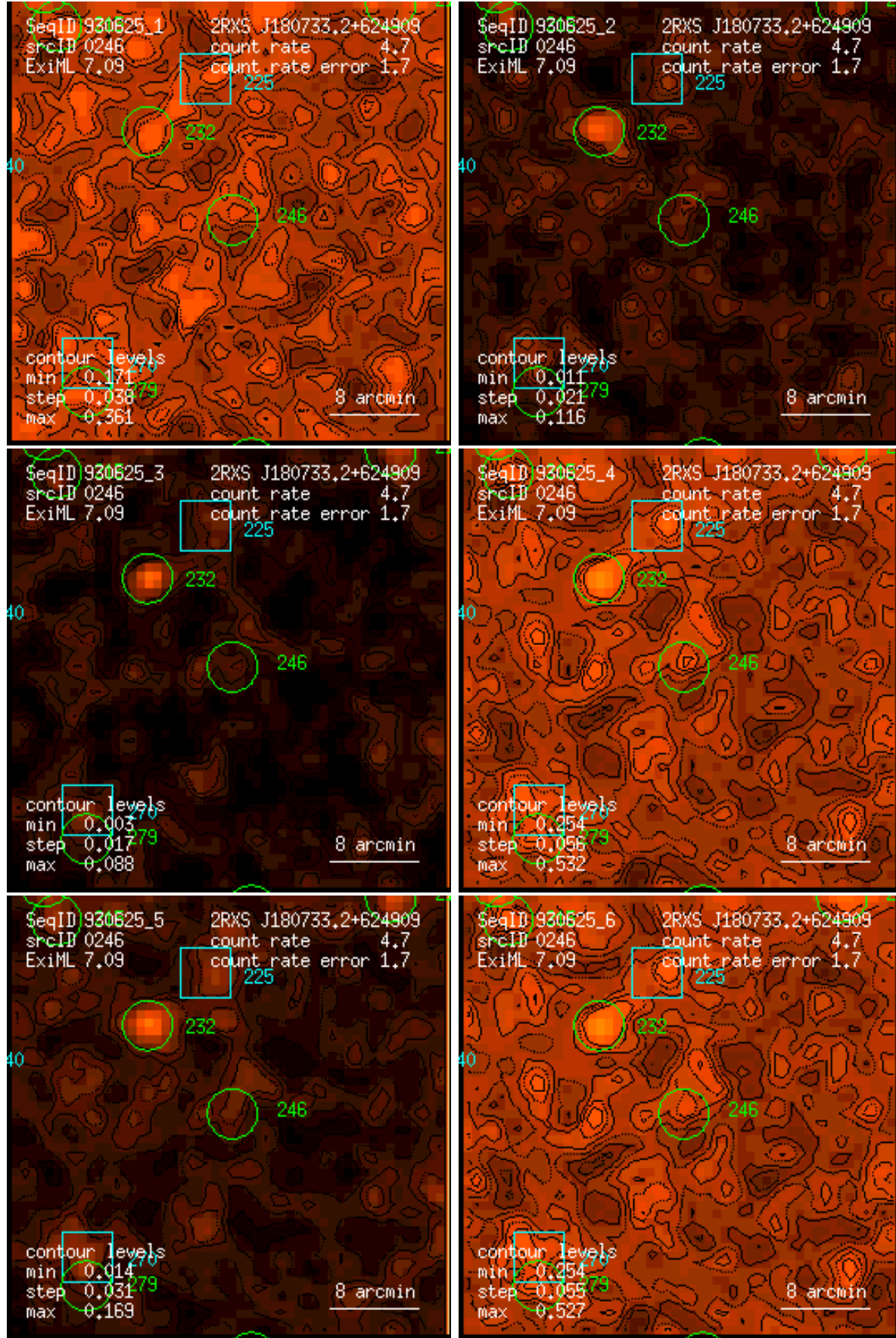
Figure 246: RASS 930625: detection 0246: band rate images, Gaussian filter: (1) PSPC channels 11 – 41, (2) 52 – 90, (3) 91 – 201, (4) 11 – 235, (5) 52 – 201, (6) 11 – 201. Broad band rates in counts/ks. Band rate contour levels in counts/ks/arcmin 2 .
