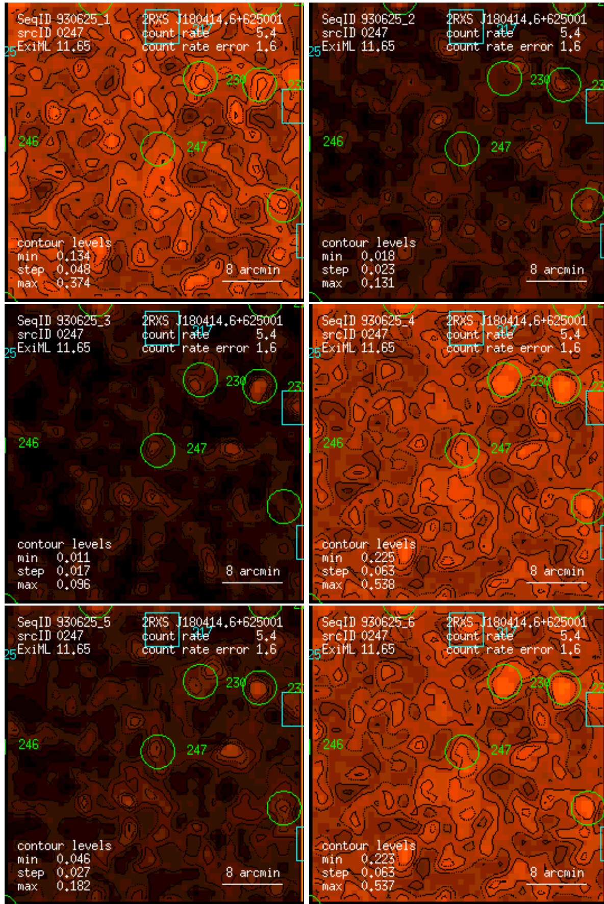
Figure 247: RASS 930625: detection 0247: band rate images, Gaussian filter: (1) PSPC channels 11 – 41, (2) 52 – 90, (3) 91 – 201, (4) 11 – 235, (5) 52 – 201, (6) 11 – 201. Broad band rates in counts/ks. Band rate contour levels in counts/ks/arcmin 2 .
