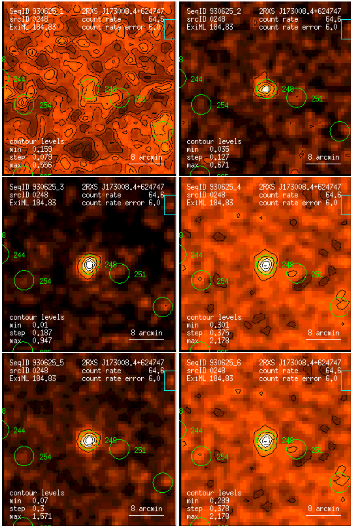
Figure 248: RASS 930625: detection 0248: band rate images, Gaussian filter: (1) PSPC channels 11 – 41, (2) 52 – 90, (3) 91 – 201, (4) 11 – 235, (5) 52 – 201, (6) 11 – 201. Broad band rates in counts/ks. Band rate contour levels in counts/ks/arcmin 2 .
