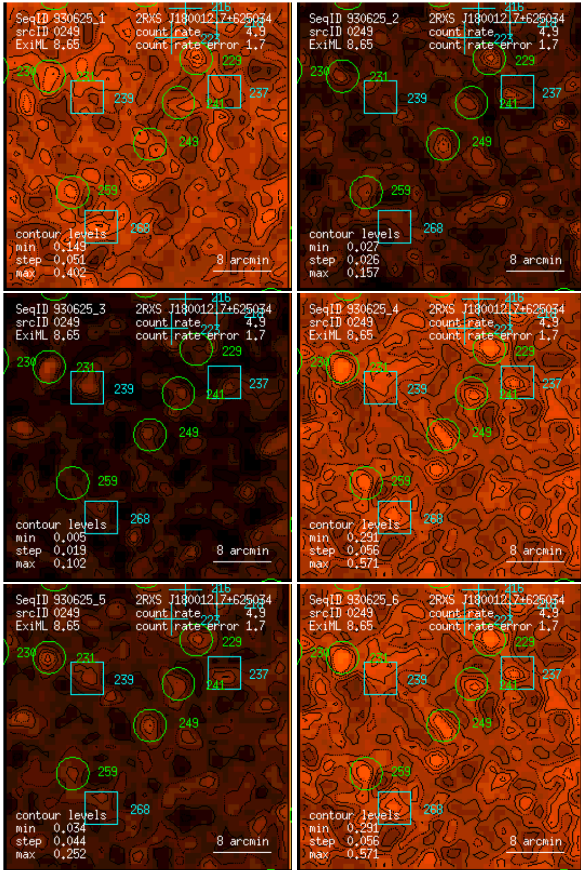
Figure 249: RASS 930625: detection 0249: band rate images, Gaussian filter: (1) PSPC channels 11 – 41, (2) 52 – 90, (3) 91 – 201, (4) 11 – 235, (5) 52 – 201, (6) 11 – 201. Broad band rates in counts/ks. Band rate contour levels in counts/ks/arcmin 2 .
