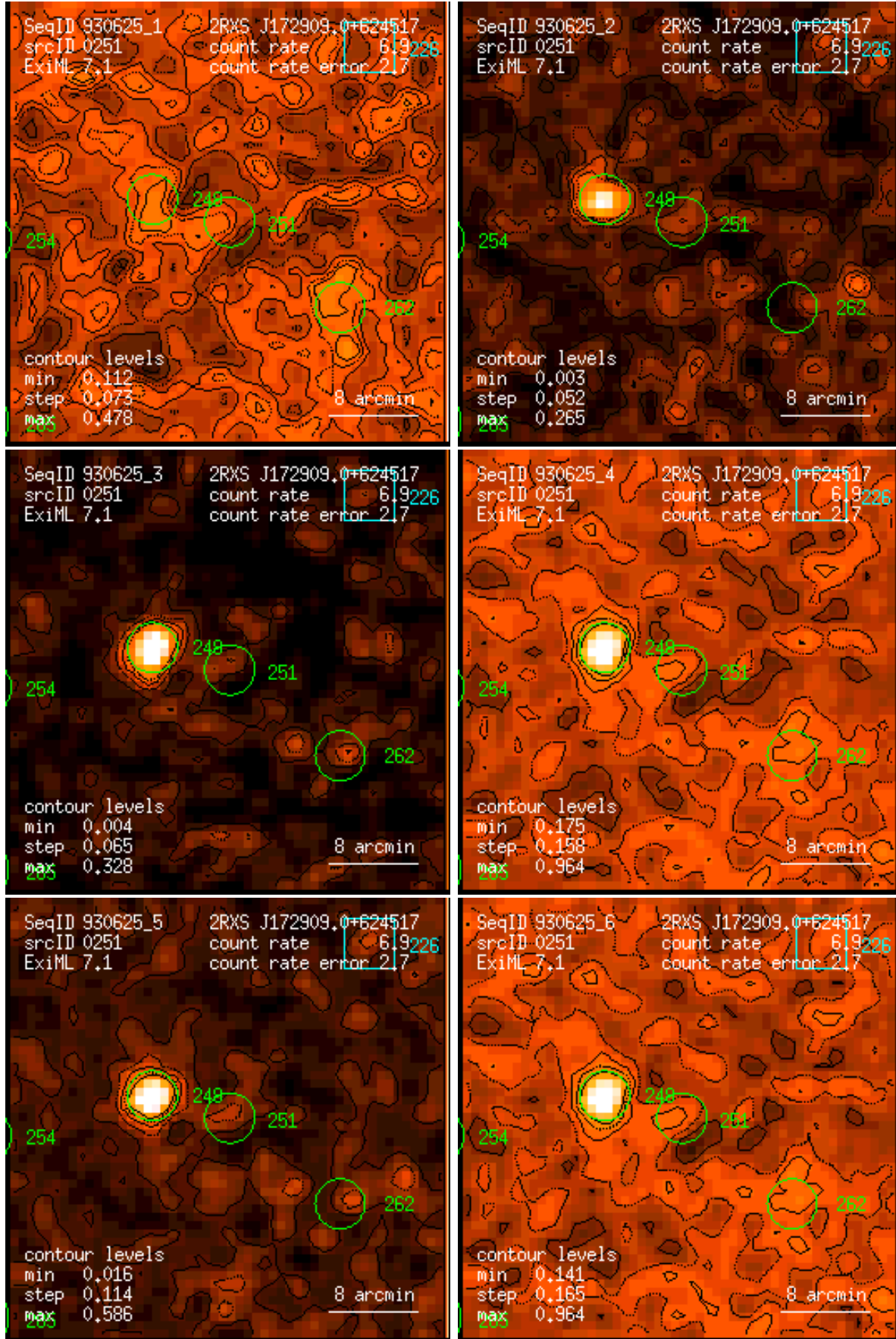
Figure 251: RASS 930625: detection 0251: band rate images, Gaussian filter: (1) PSPC channels 11 – 41, (2) 52 – 90, (3) 91 – 201, (4) 11 – 235, (5) 52 – 201, (6) 11 – 201. Broad band rates in counts/ks. Band rate contour levels in counts/ks/arcmin 2 .
