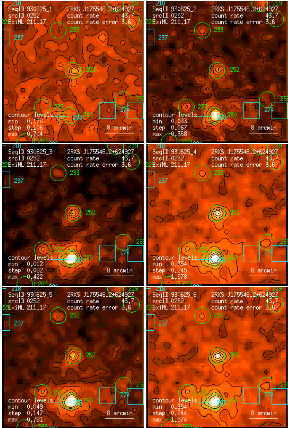
Figure 252: RASS 930625: detection 0252: band rate images, Gaussian filter: (1) PSPC channels 11 – 41, (2) 52 – 90, (3) 91 – 201, (4) 11 – 235, (5) 52 – 201, (6) 11 – 201. Broad band rates in counts/ks. Band rate contour levels in counts/ks/arcmin 2 .
