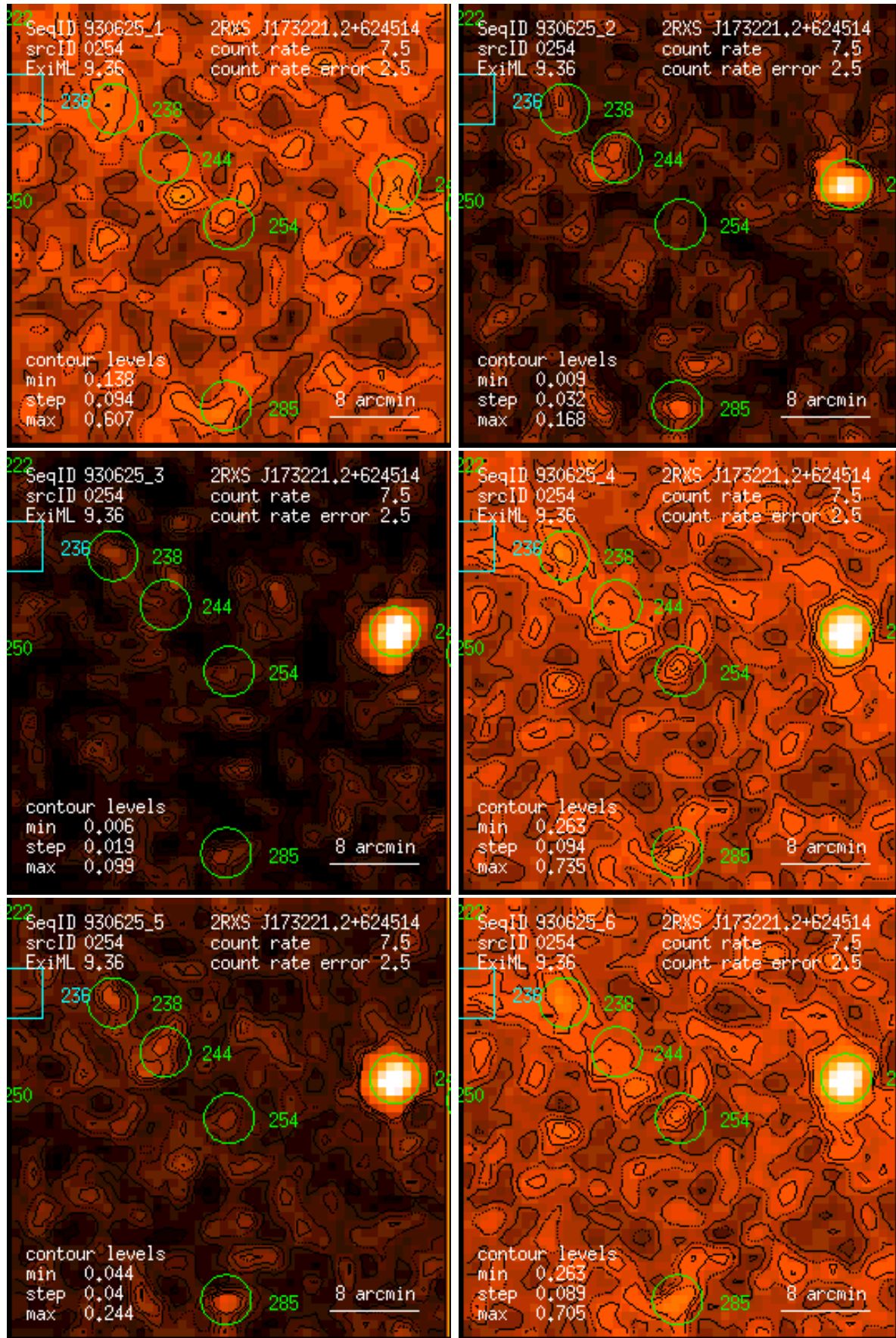
Figure 254: RASS 930625: detection 0254: band rate images, Gaussian filter: (1) PSPC channels 11 – 41, (2) 52 – 90, (3) 91 – 201, (4) 11 – 235, (5) 52 – 201, (6) 11 – 201. Broad band rates in counts/ks. Band rate contour levels in counts/ks/arcmin 2 .
