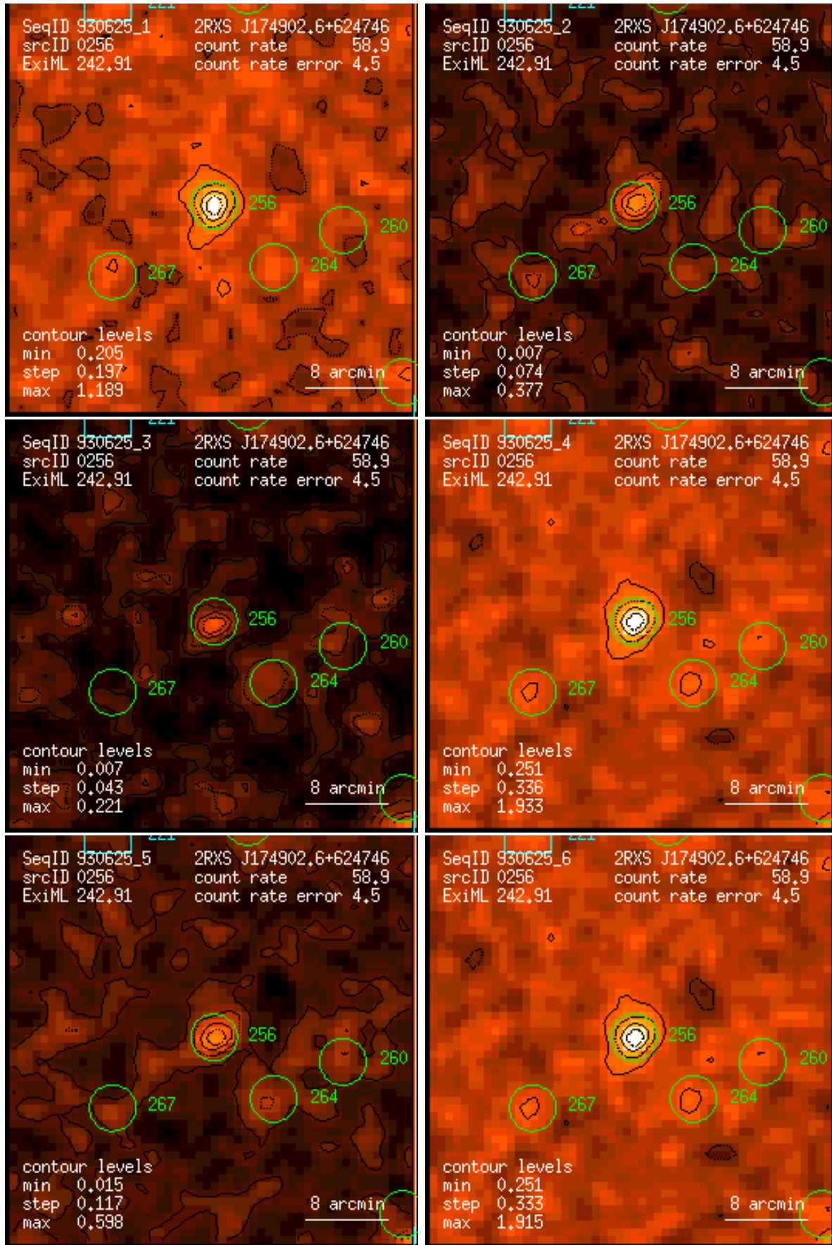
Figure 256: RASS 930625: detection 0256: band rate images, Gaussian filter: (1) PSPC channels 11 – 41, (2) 52 – 90, (3) 91 – 201, (4) 11 – 235, (5) 52 – 201, (6) 11 – 201. Broad band rates in counts/ks. Band rate contour levels in counts/ks/arcmin 2 .
