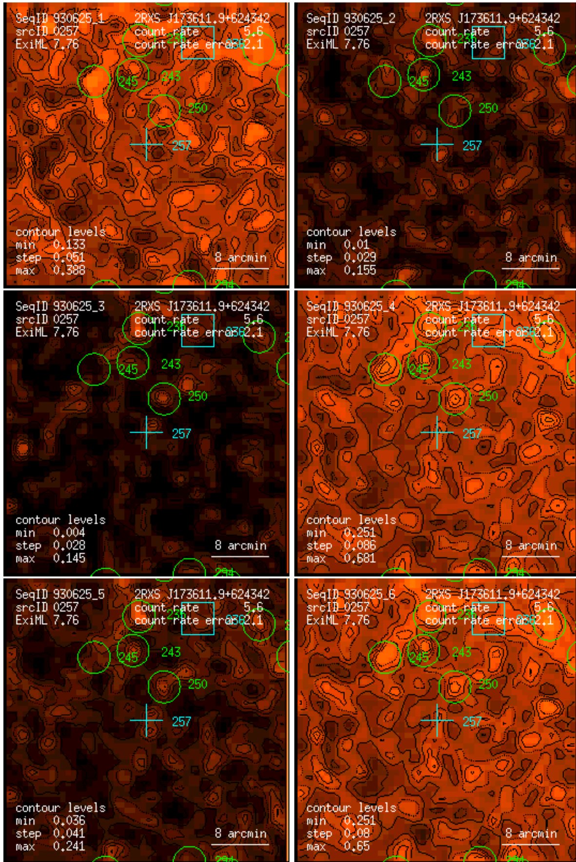
Figure 257: RASS 930625: detection 0257: band rate images, Gaussian filter: (1) PSPC channels 11 – 41, (2) 52 – 90, (3) 91 – 201, (4) 11 – 235, (5) 52 – 201, (6) 11 – 201. Broad band rates in counts/ks. Band rate contour levels in counts/ks/arcmin 2 .
