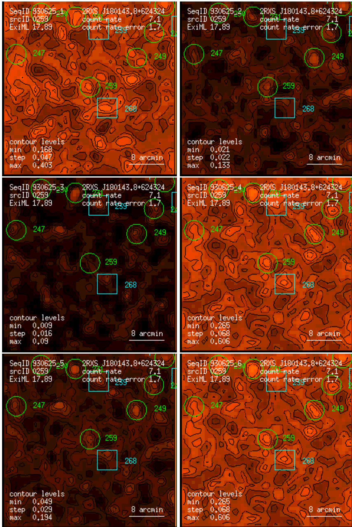
Figure 259: RASS 930625: detection 0259: band rate images, Gaussian filter: (1) PSPC channels 11 – 41, (2) 52 – 90, (3) 91 – 201, (4) 11 – 235, (5) 52 – 201, (6) 11 – 201. Broad band rates in counts/ks. Band rate contour levels in counts/ks/arcmin 2 .
