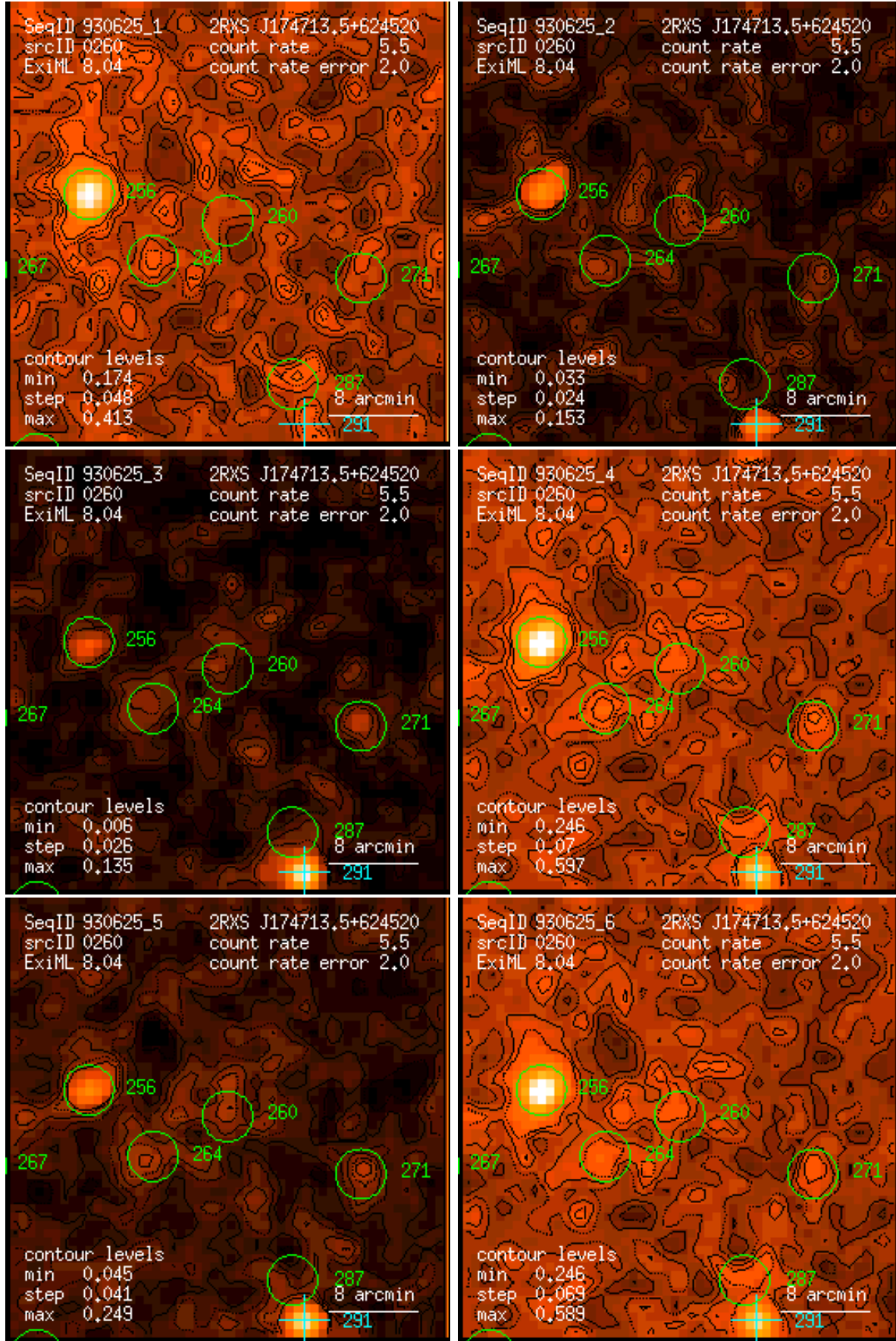
Figure 260: RASS 930625: detection 0260: band rate images, Gaussian filter: (1) PSPC channels 11 – 41, (2) 52 – 90, (3) 91 – 201, (4) 11 – 235, (5) 52 – 201, (6) 11 – 201. Broad band rates in counts/ks. Band rate contour levels in counts/ks/arcmin 2 .
