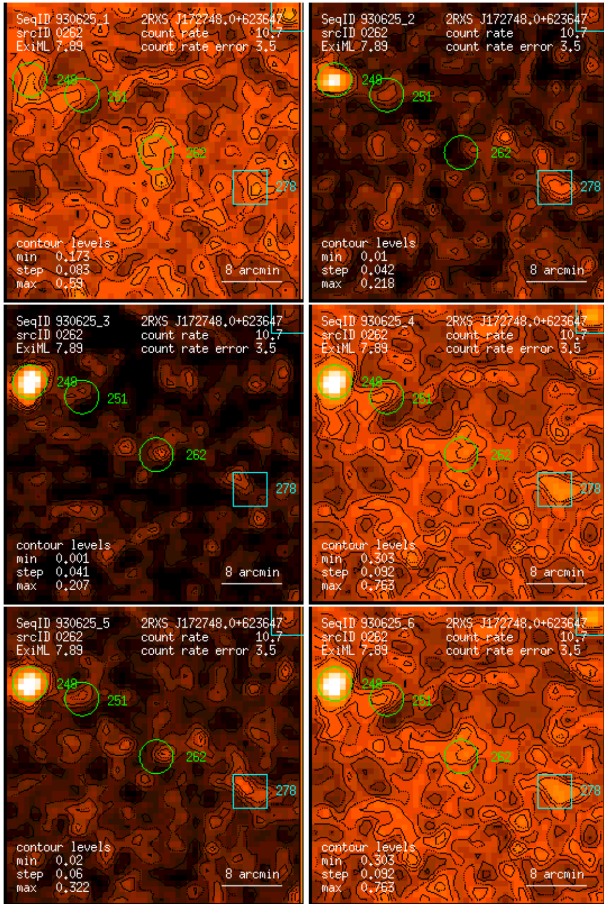
Figure 262: RASS 930625: detection 0262: band rate images, Gaussian filter: (1) PSPC channels 11 – 41, (2) 52 – 90, (3) 91 – 201, (4) 11 – 235, (5) 52 – 201, (6) 11 – 201. Broad band rates in counts/ks. Band rate contour levels in counts/ks/arcmin 2 .
