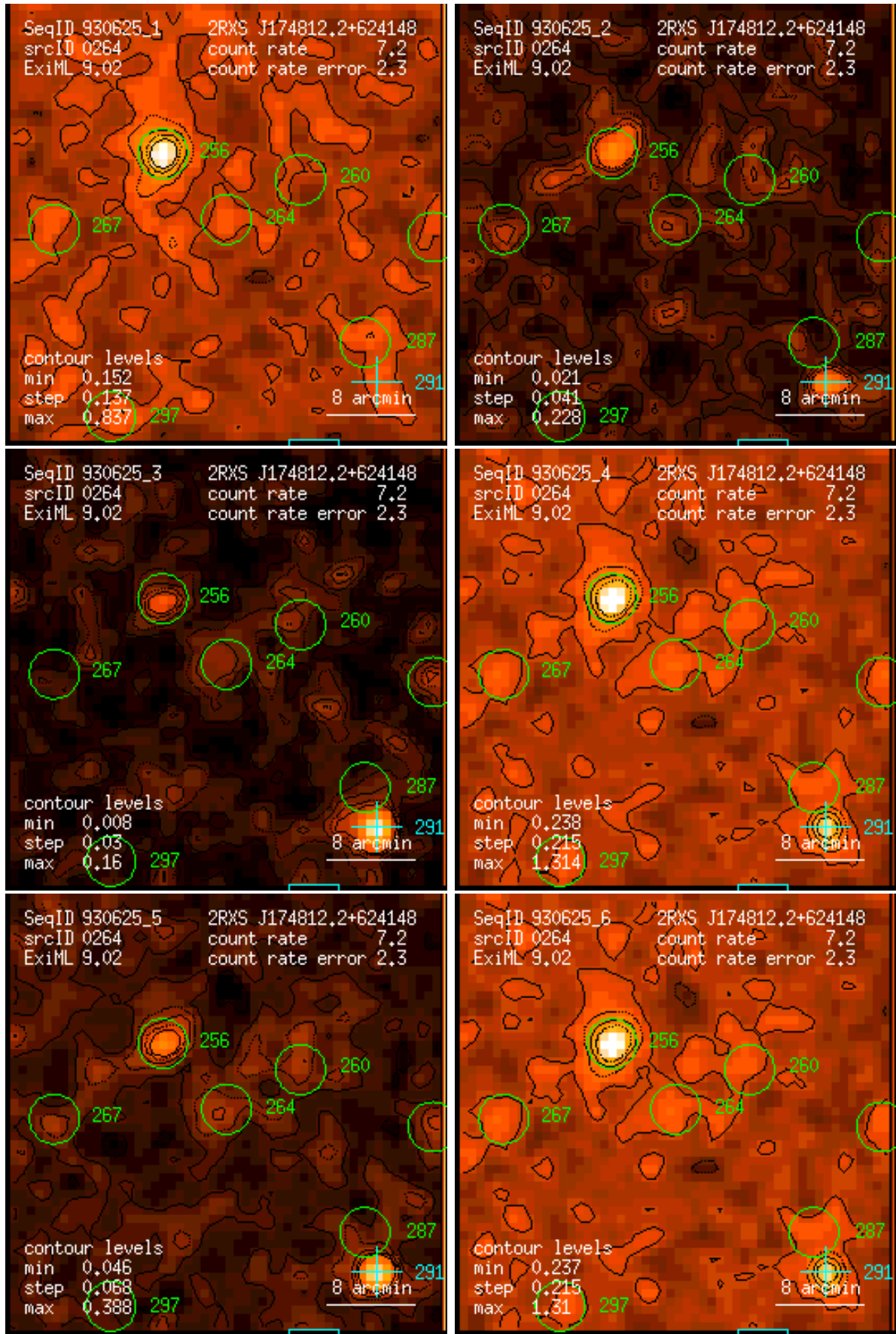
Figure 264: RASS 930625: detection 0264: band rate images, Gaussian filter: (1) PSPC channels 11 – 41, (2) 52 – 90, (3) 91 – 201, (4) 11 – 235, (5) 52 – 201, (6) 11 – 201. Broad band rates in counts/ks. Band rate contour levels in counts/ks/arcmin 2 .
