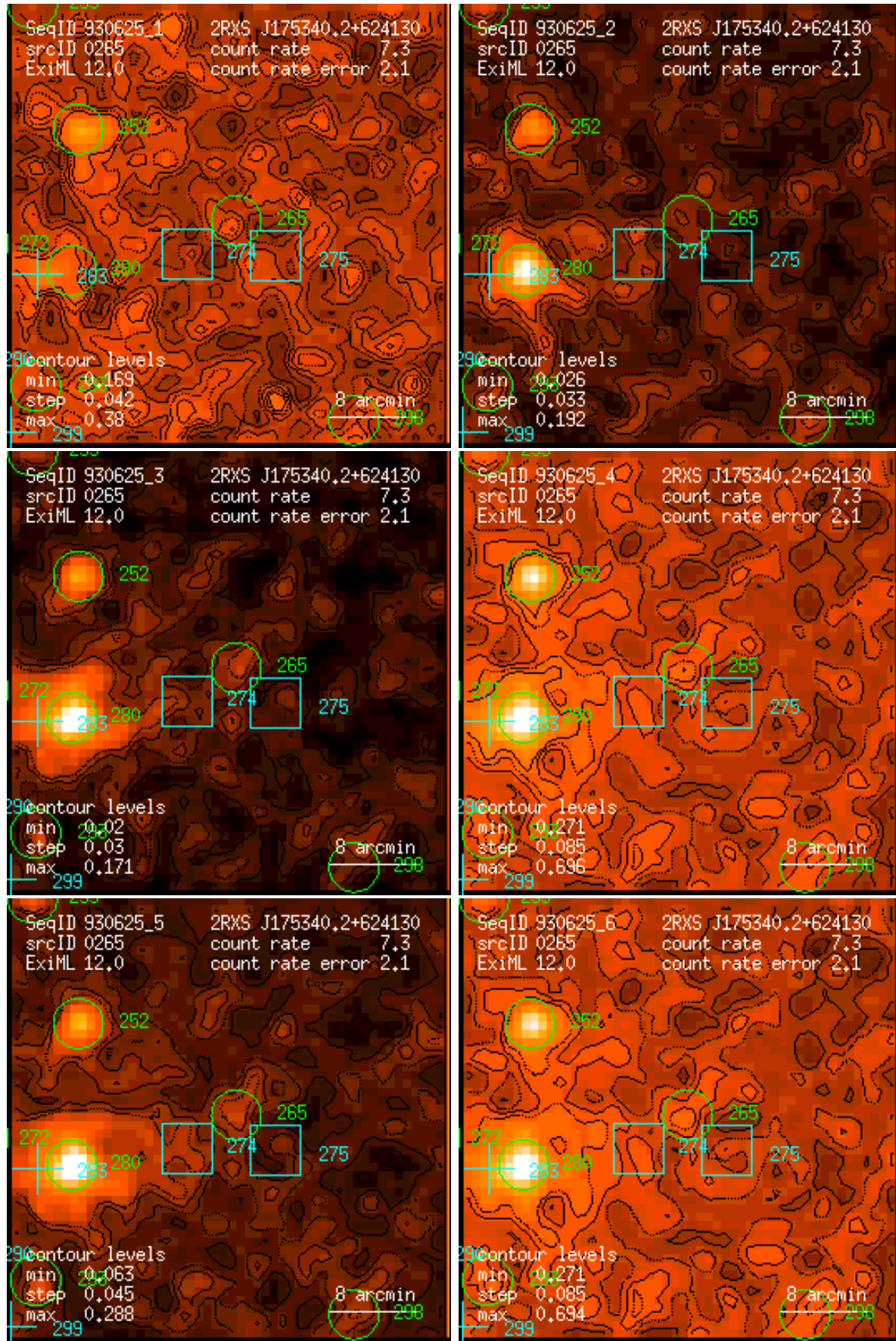
Figure 265: RASS 930625: detection 0265: band rate images, Gaussian filter: (1) PSPC channels 11 – 41, (2) 52 – 90, (3) 91 – 201, (4) 11 – 235, (5) 52 – 201, (6) 11 – 201. Broad band rates in counts/ks. Band rate contour levels in counts/ks/arcmin 2 .
