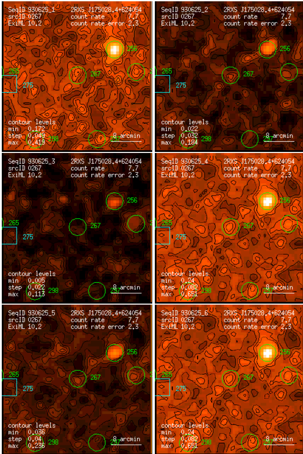
Figure 267: RASS 930625: detection 0267: band rate images, Gaussian filter: (1) PSPC channels 11 – 41, (2) 52 – 90, (3) 91 – 201, (4) 11 – 235, (5) 52 – 201, (6) 11 – 201. Broad band rates in counts/ks. Band rate contour levels in counts/ks/arcmin 2 .
