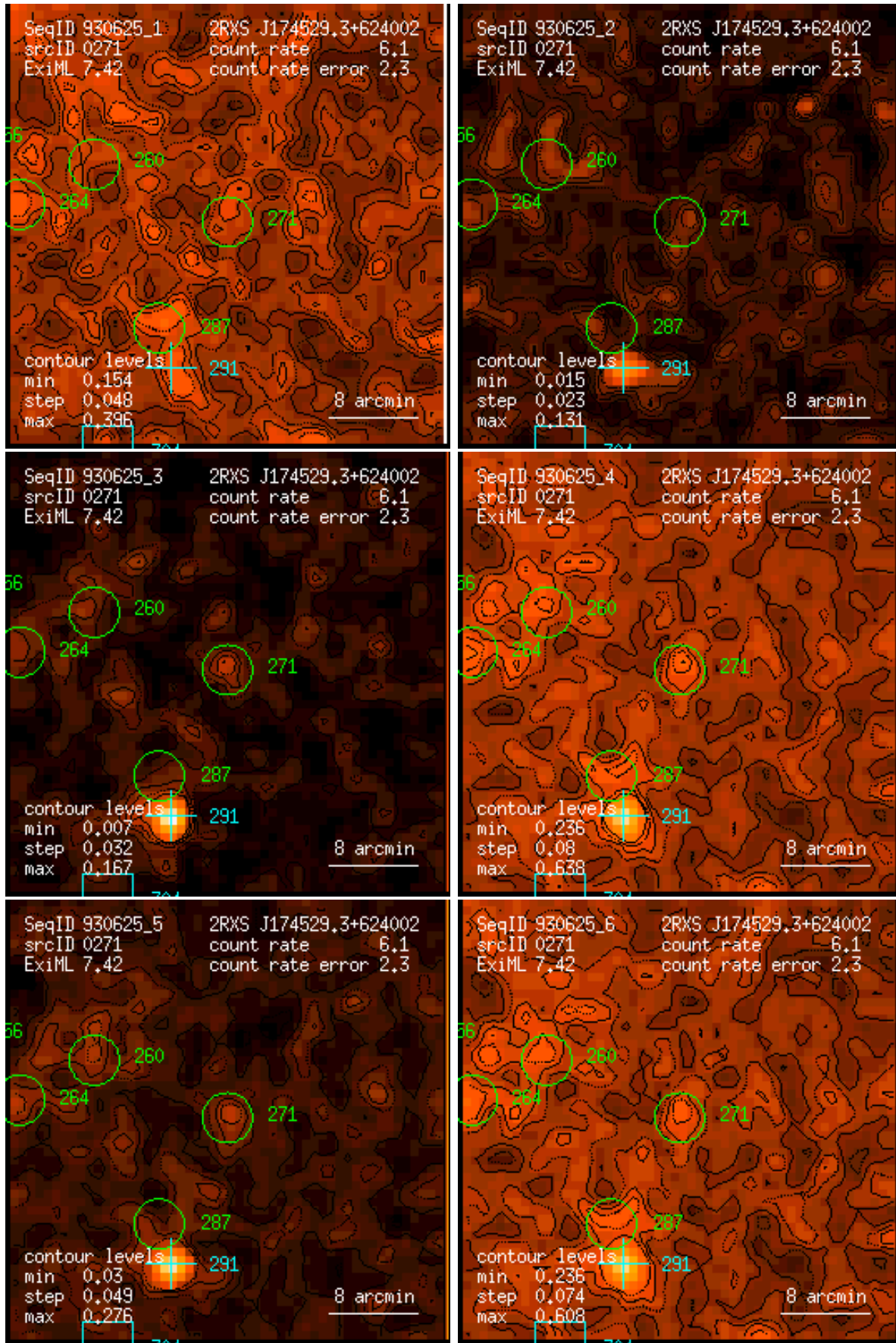
Figure 271: RASS 930625: detection 0271: band rate images, Gaussian filter: (1) PSPC channels 11 – 41, (2) 52 – 90, (3) 91 – 201, (4) 11 – 235, (5) 52 – 201, (6) 11 – 201. Broad band rates in counts/ks. Band rate contour levels in counts/ks/arcmin 2 .
