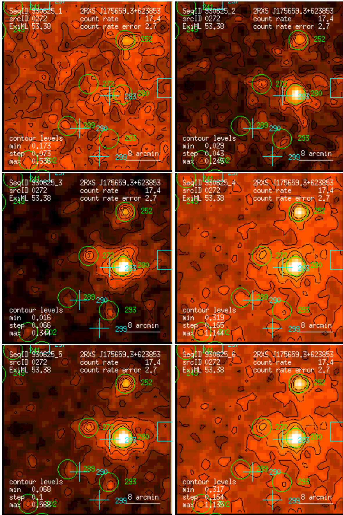
Figure 272: RASS 930625: detection 0272: band rate images, Gaussian filter: (1) PSPC channels 11 – 41, (2) 52 – 90, (3) 91 – 201, (4) 11 – 235, (5) 52 – 201, (6) 11 – 201. Broad band rates in counts/ks. Band rate contour levels in counts/ks/arcmin 2 .
