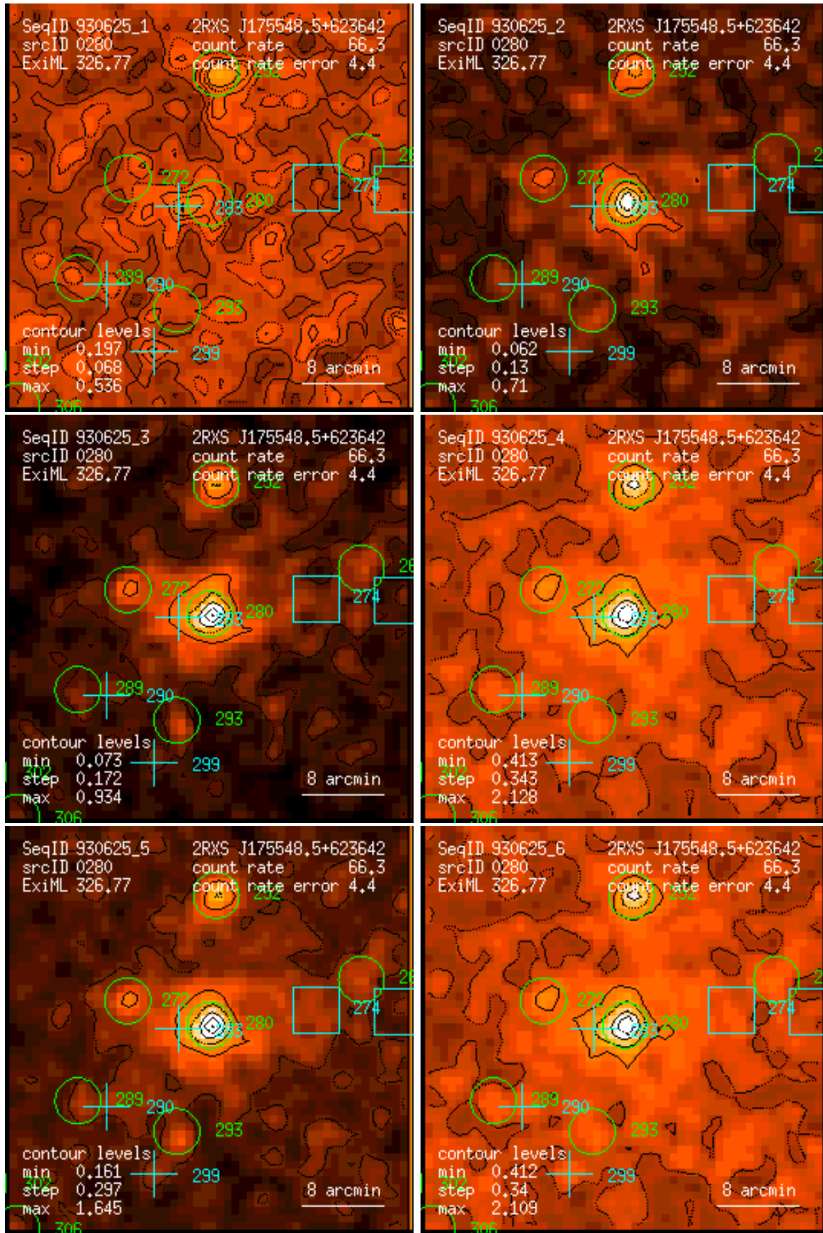
Figure 280: RASS 930625: detection 0280: band rate images, Gaussian filter: (1) PSPC channels 11 – 41, (2) 52 – 90, (3) 91 – 201, (4) 11 – 235, (5) 52 – 201, (6) 11 – 201. Broad band rates in counts/ks. Band rate contour levels in counts/ks/arcmin 2 .
