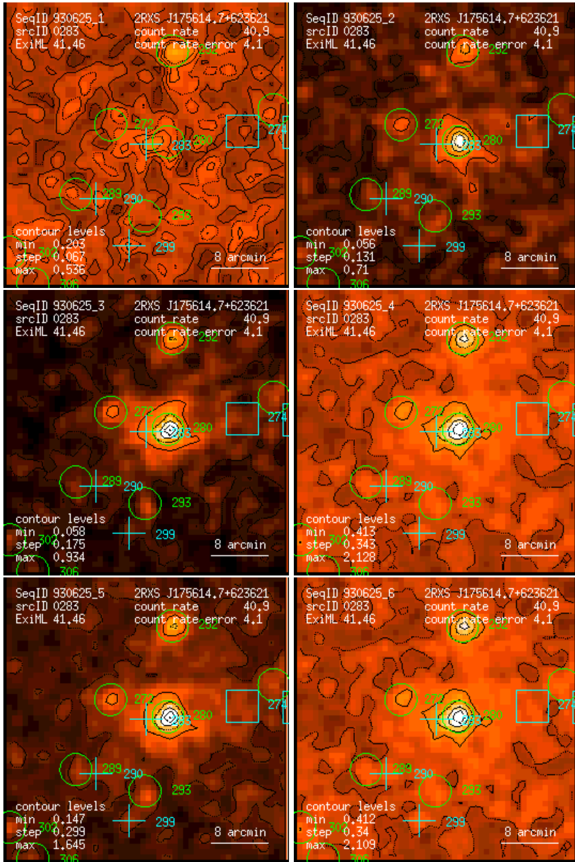
Figure 283: RASS 930625: detection 0283: band rate images, Gaussian filter: (1) PSPC channels 11 – 41, (2) 52 – 90, (3) 91 – 201, (4) 11 – 235, (5) 52 – 201, (6) 11 – 201. Broad band rates in counts/ks. Band rate contour levels in counts/ks/arcmin 2 .
