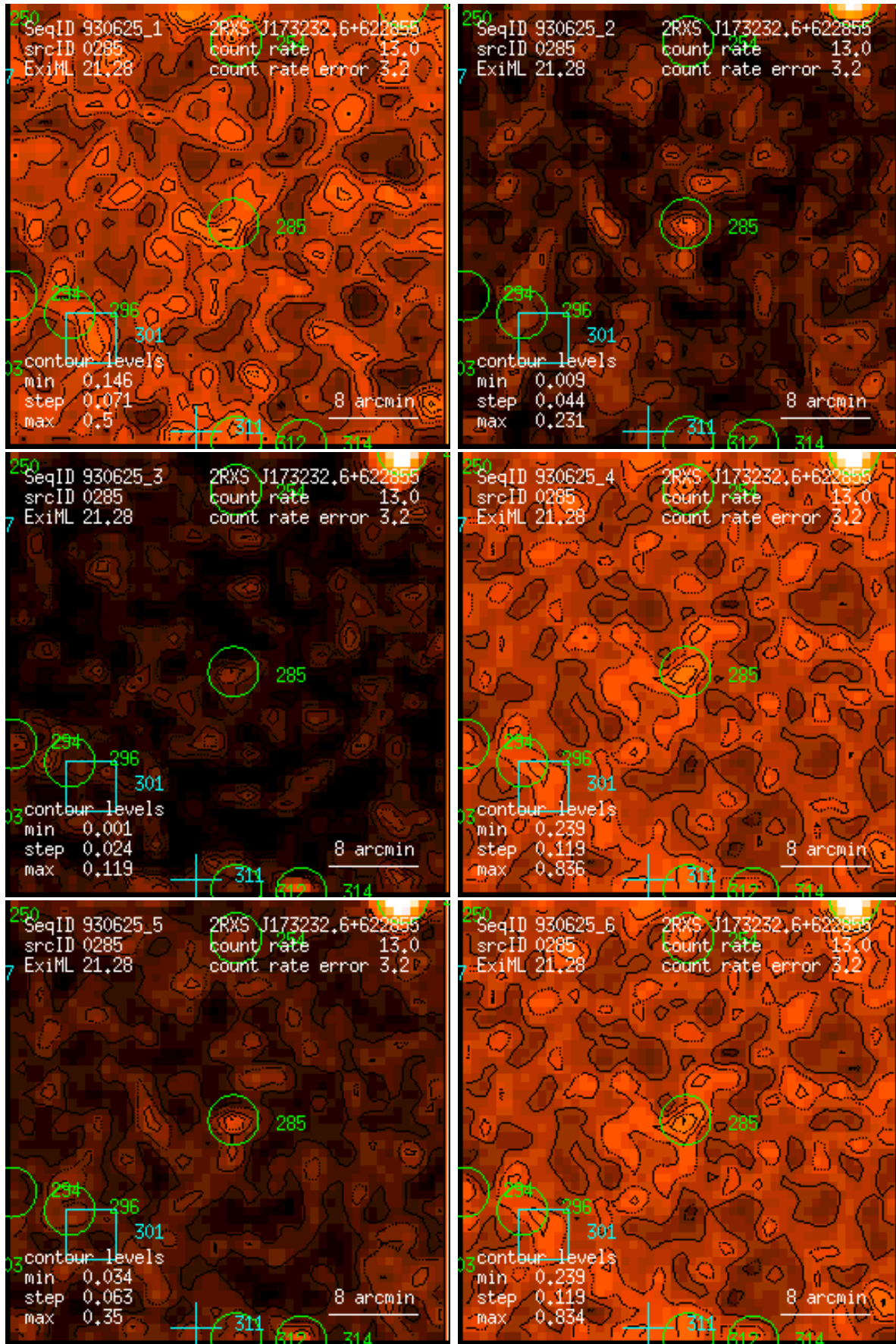
Figure 285: RASS 930625: detection 0285: band rate images, Gaussian filter: (1) PSPC channels 11 – 41, (2) 52 – 90, (3) 91 – 201, (4) 11 – 235, (5) 52 – 201, (6) 11 – 201. Broad band rates in counts/ks. Band rate contour levels in counts/ks/arcmin 2 .
