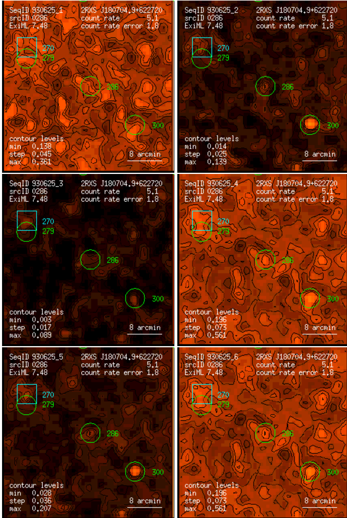
Figure 286: RASS 930625: detection 0286: band rate images, Gaussian filter: (1) PSPC channels 11 – 41, (2) 52 – 90, (3) 91 – 201, (4) 11 – 235, (5) 52 – 201, (6) 11 – 201. Broad band rates in counts/ks. Band rate contour levels in counts/ks/arcmin 2 .
