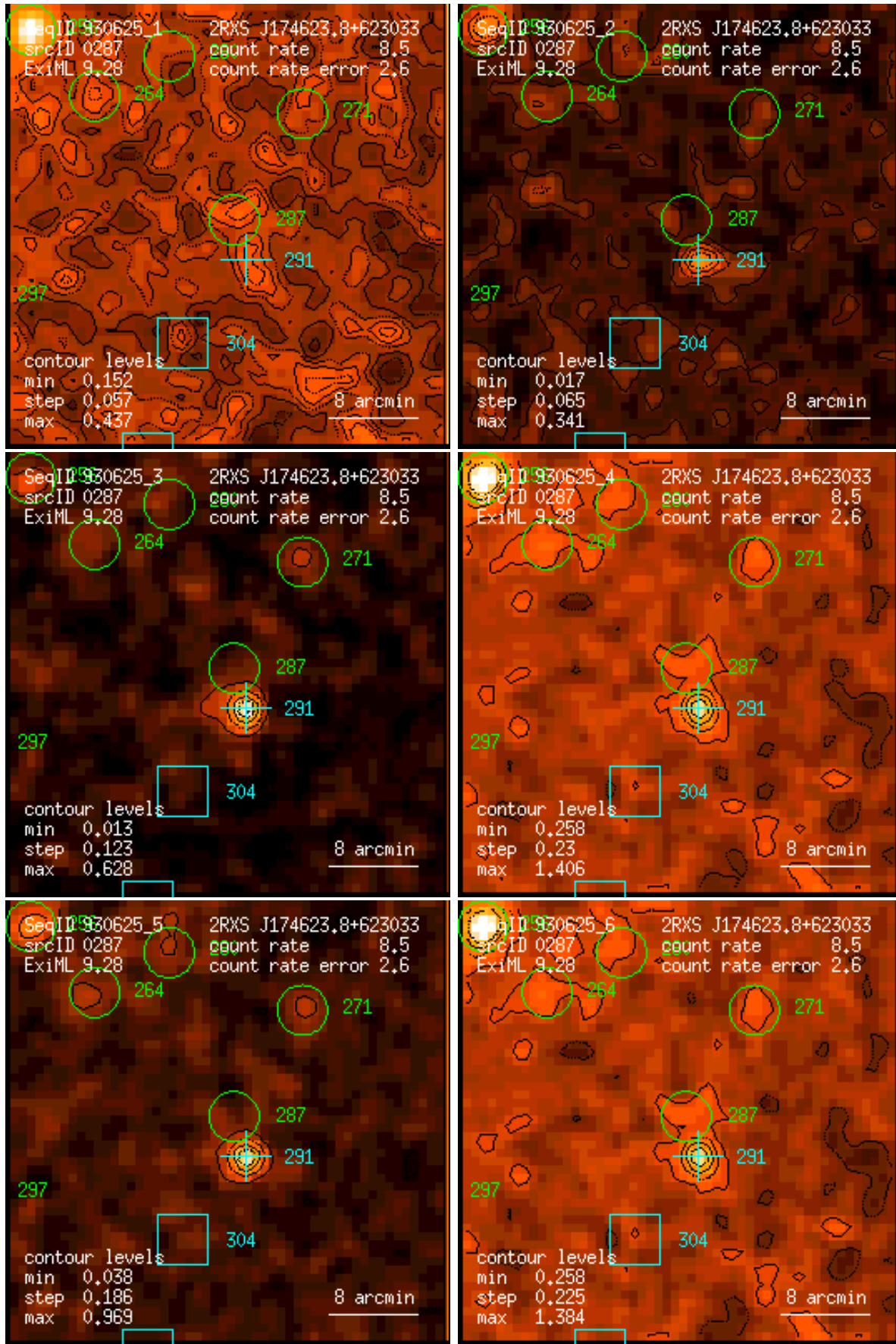
Figure 287: RASS 930625: detection 0287: band rate images, Gaussian filter: (1) PSPC channels 11 – 41, (2) 52 – 90, (3) 91 – 201, (4) 11 – 235, (5) 52 – 201, (6) 11 – 201. Broad band rates in counts/ks. Band rate contour levels in counts/ks/arcmin 2 .
