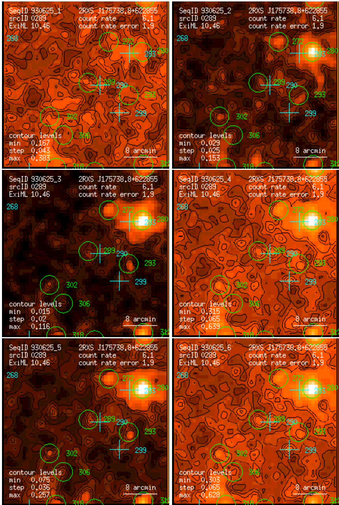
Figure 289: RASS 930625: detection 0289: band rate images, Gaussian filter: (1) PSPC channels 11 – 41, (2) 52 – 90, (3) 91 – 201, (4) 11 – 235, (5) 52 – 201, (6) 11 – 201. Broad band rates in counts/ks. Band rate contour levels in counts/ks/arcmin 2 .
