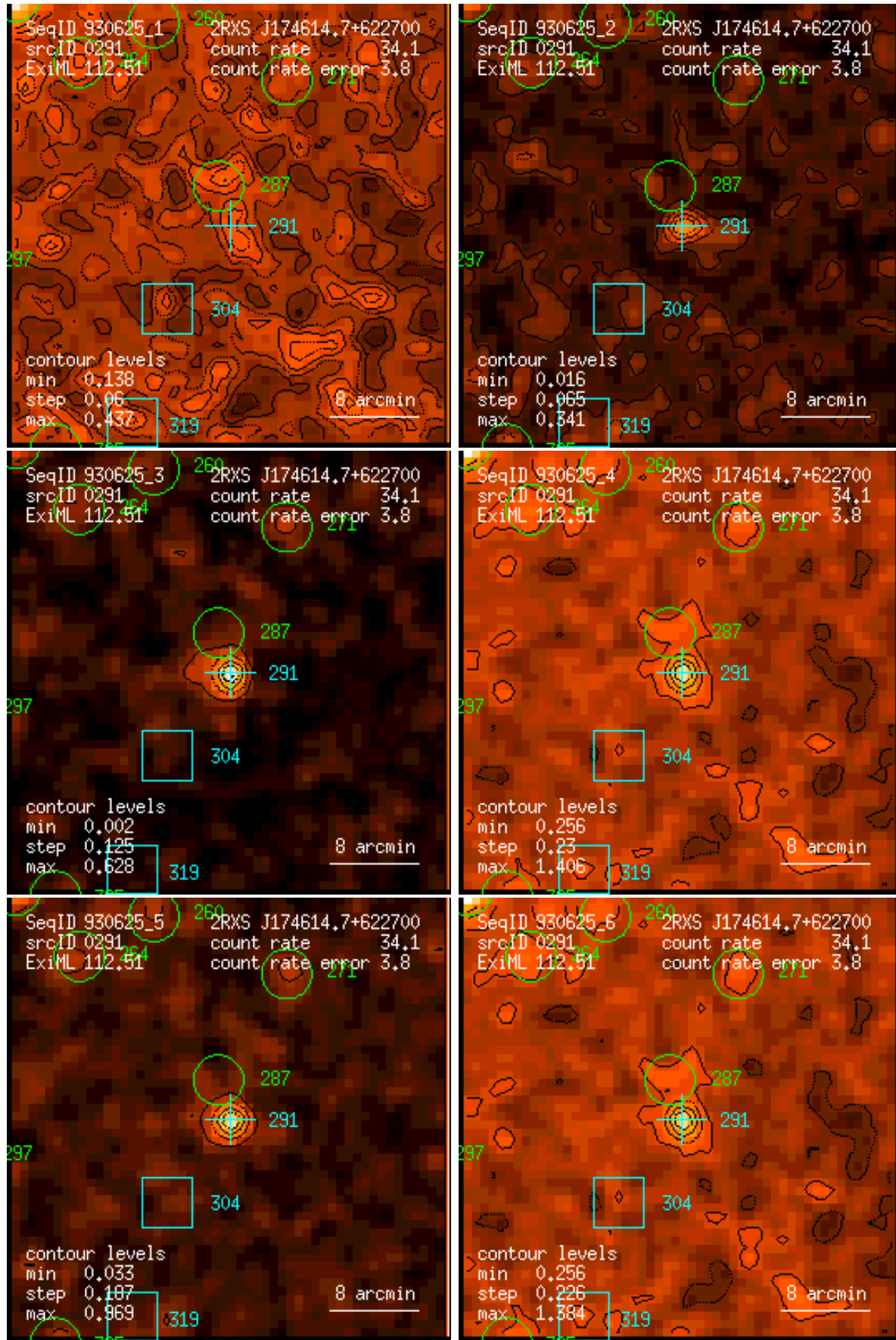
Figure 291: RASS 930625: detection 0291: band rate images, Gaussian filter: (1) PSPC channels 11 – 41, (2) 52 – 90, (3) 91 – 201, (4) 11 – 235, (5) 52 – 201, (6) 11 – 201. Broad band rates in counts/ks. Band rate contour levels in counts/ks/arcmin 2 .
