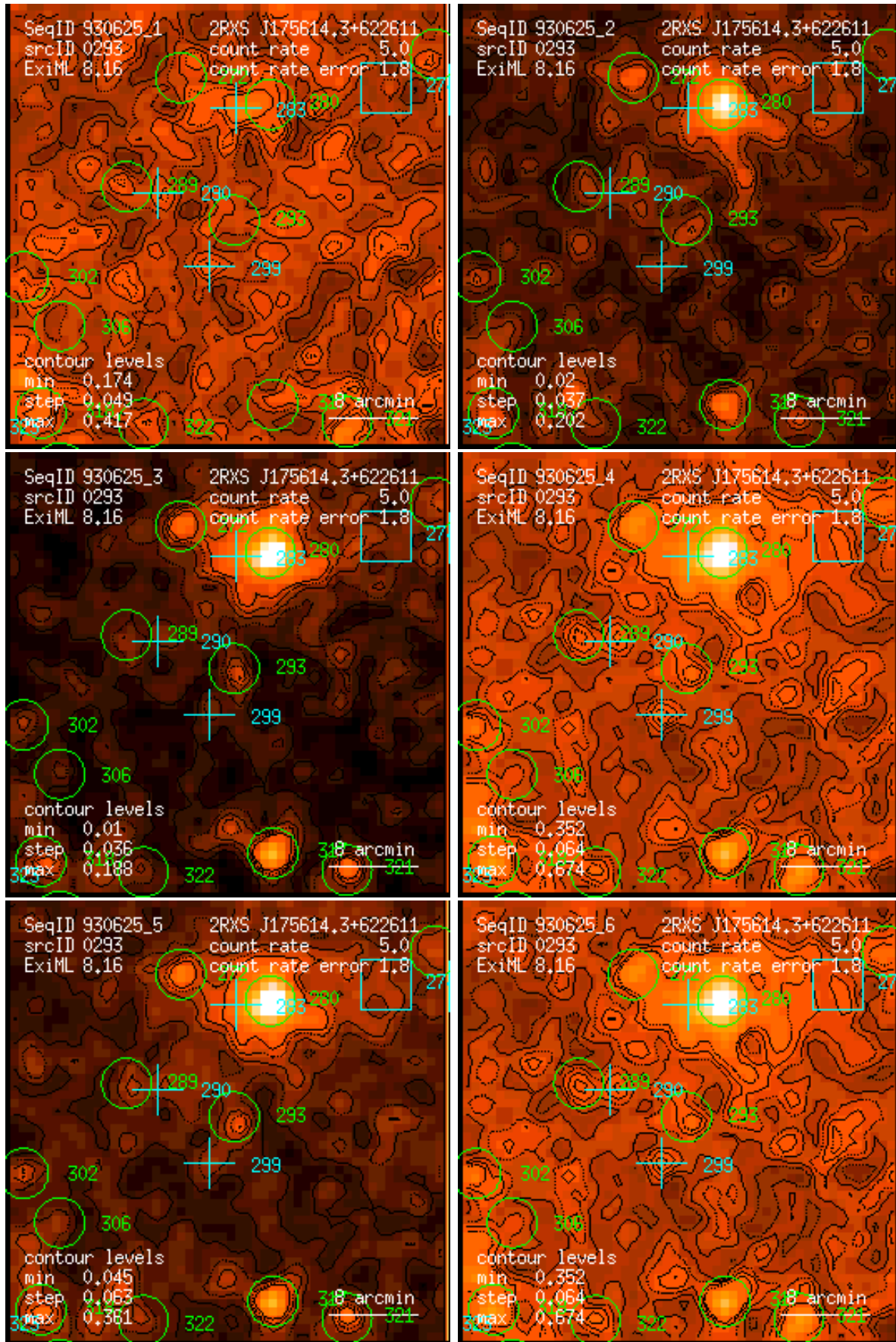
Figure 293: RASS 930625: detection 0293: band rate images, Gaussian filter: (1) PSPC channels 11 – 41, (2) 52 – 90, (3) 91 – 201, (4) 11 – 235, (5) 52 – 201, (6) 11 – 201. Broad band rates in counts/ks. Band rate contour levels in counts/ks/arcmin 2 .
